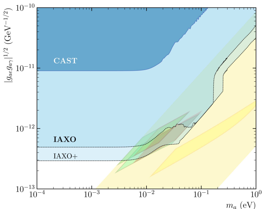
Figure 3. Sensitivity plot of IAXO to BCA ( g_{ae} -mediated) solar axions, in the (|g_{ae}g_{a\gamma}|^{1/2}-m_a) parameter space. The yellow band corresponds to the QCD axion models and the diamond-shaped color regions correspond to particular QCD axion models that are able to fit all the anomalous stellar cooling observations, following [23].
