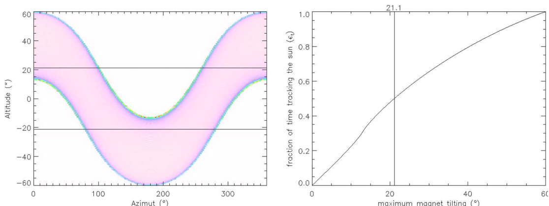
Figure 44. Left: region of the azimuth-altitude coordinates of the Sun position along the year for DESY geographical coordinates. The horizontal lines correspond to an elevation of \pm 21.1^\circ . Right: fraction of the time the Sun is reachable versus maximum elevation. The horizontal line indicates that an elevation of \pm 21.1^\circ would correspond to a 50 % of average exposure over the year.
