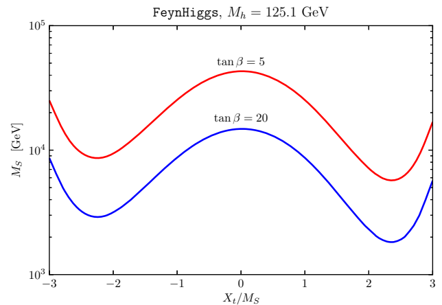
Fig. 2 Values of the SUSY mass parameter M_S and of the stop mixing parameter X_t (normalized to M_S ) that lead to the prediction M_h = 125.1 \text{ GeV} , in a simplified MSSM scenario with degenerate SUSY masses, for \tan \beta = 20 (blue) or \tan \beta = 5 (red)
