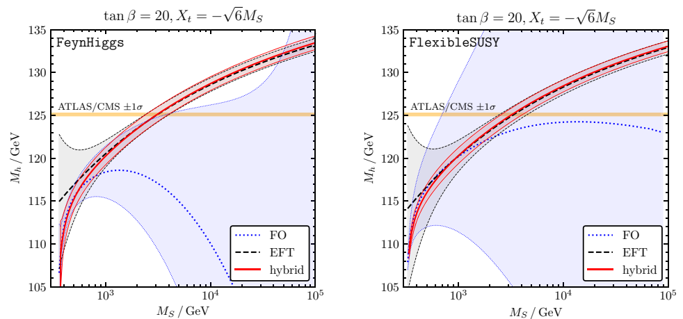
Fig. 5 Comparison between the pure FO, pure EFT and hybrid calculations of the Higgs mass, with the corresponding estimates of the theory uncertainty, in an MSSM scenario with degenerate SUSY masses. The sfermion mass and mixing parameters are defined in the \overline{\text{DR}} scheme at the scale Q = M_S . The left plot is produced with FeynHiggs, the right one with different modules of FlexibleSUSY
