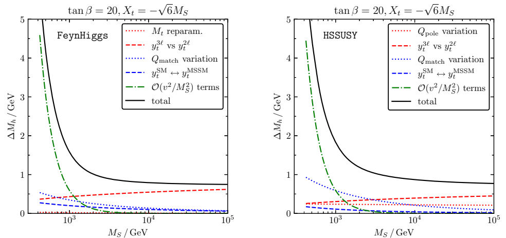
Fig. 4 Estimates of the different sources of theory uncertainty for the EFT calculation, as a function of the SUSY scale M_S . The left plot is produced with FeynHiggs, the right one with HSSUSY
