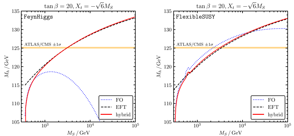
Fig. 3 Comparison between the pure FO, pure EFT and hybrid calculations of the mass of the SM-like Higgs boson in an MSSM scenario with degenerate SUSY masses. The sfermion mass and mixing parameters are defined in the \overline{\text{DR}} scheme at the scale Q = M_S . The left plot is produced with FeynHiggs, the right one with different modules of FlexibleSUSY
