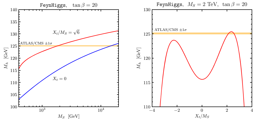
Fig. 1 The lighter CP-even Higgs mass in the MSSM as a function of a common SUSY mass parameter M_S and of the stop mixing parameter X_t (normalized to M_S ). Both parameters are defined in the \overline{\text{DR}} scheme at the scale Q = M_S
