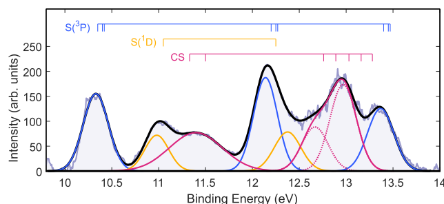
FIG. 4. Deconvolution of the scaled background subtracted photoelectron spectrum used to obtain the S(^3P)/S(^1D) branching ratio. The black line represents the total fit to the scaled background subtracted spectrum, which is plotted as a pale blue line. The individual Gaussian contributions to the overall fit are also plotted and color-coded to match the color of the combs.
