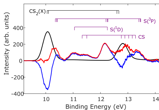
FIG. 1. Photoelectron spectrum obtained from ionization of the electronic ground state of \text{CS}_2 (black). The two peaks correspond to ionization into the ground and A states of the cation. Background subtracted photoelectron spectrum obtained after dissociation is complete, following the subtraction of the full background intensity (blue) and subtraction of a scaled version of the background equivalent to the unpumped ground state population (red). Combs above the spectra mark the expected positions of photoelectron bands based on the known ionization potentials.
