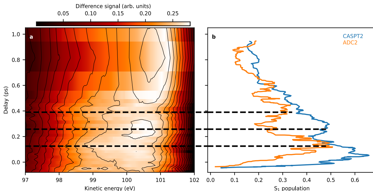
Fig. 3 Experimental shifts and theoretical predictions on state population. a False-colour contour plot of the positive lobe in Fig. 2b, normalised on the time-dependent area under the lobe. An oscillatory dynamic in the lineshape and position is visible for the first ~600 fs. At 150 fs and 400 fs delay, the spectrum is shifted to lower kinetic energy, while it is shifted to higher kinetic energies in between and afterwards. b Comparison of the oscillation dynamics with trajectory simulations. The population of the S_1 ( n\pi^* ) state, obtained from CASPT2 calculations of Ref. 35 (blue line) and ADC(2) calculations of Ref. 36 (orange line) are plotted. The dashed lines highlight the extrema of the oscillation observed in the experiment. The theoretical simulations do not include finite time-resolution and we shifted them by 50 fs to smaller delays to induce a transient rise of the signal around zero delay. The experimental 250 fs oscillation features have their counterparts in the simulated S_1 population, indicating the observation of a population exchange between the S_1 state and other electronic states. Source Data (for a) are provided as Source Data file.
