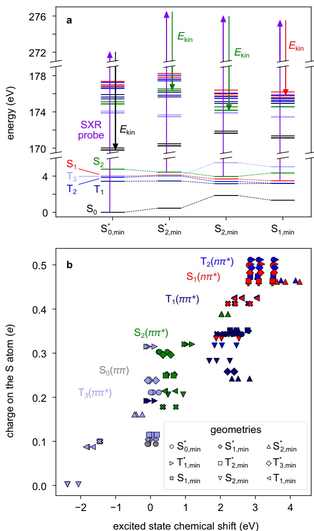
Fig. 4 Soft x-ray photoelectron probing of the excited-state dynamics of 2-thiouracil in a multi-electron picture. a Calculated electronic energies of the valence excited states, in the range 0–6 eV, and the core ionised states, in the range of 170–179 eV, for four geometries relevant in the short time dynamics. The arrows illustrate the 2p -1 ionisation process associated with the most intense transition. The core ionised states are grouped into sets of three states, which follow the colour coding of the valence states, meaning that their valence configuration is maintained with a 2p x , 2p y or 2p z core hole. Accordingly, the electron kinetic energy E_{\text{kin}} refers to ionisations out of S 0 , S 1 ( n\pi^* ) and S 2 ( \pi\pi^* ), depending on the geometry. b Partial charges on the S atom are plotted against the excited state chemical shift of the 2p electrons, calculated for the valence states at nine different geometries. For each geometry, the graph includes three markers for each excited state (S 1 , S 2 , T 1 , T 2 , T 3 ); in addition, three dots are included for the ionisation from S 0 at S 0,min , for a total of 9 \times 3 \times 5 + 3 = 138 markers. Asterisks denote restriction in the calculation of the states to planar geometries. Source Data are provided as a Source Data file.
