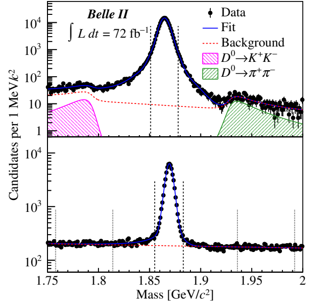
Figure 1: Mass distributions of (top) D^0 \rightarrow K^-\pi^+ and (bottom) D^+ \rightarrow K^-\pi^+\pi^+ candidates with fit projections overlaid. The vertical dashed and (for the bottom plot) dotted lines indicate the signal regions and the sideband, respectively.
