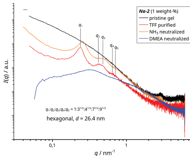
Fig. 8 SAXS of Na-2, the pristine, diluted gel and of dispersions of the TFF-purified nano-ribbons: tel-quel as well as \text{NH}_3 and DMEA neutralized (all 1 weight-%).
