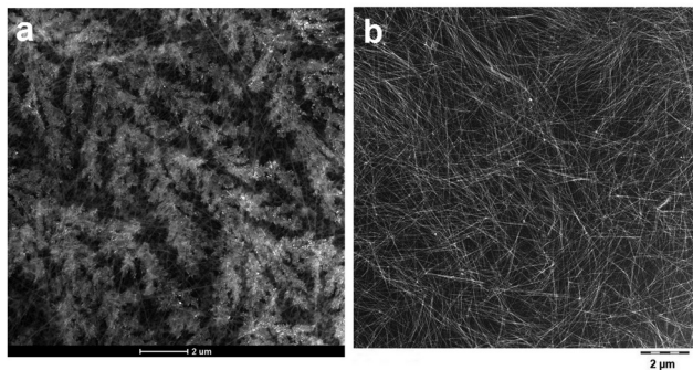
Fig. 2 High angle annular dark field (HAADF) TEM image of (a) Na-2 and (b) sediment phase of Na-2. Scale bars are 2 \mu m.
