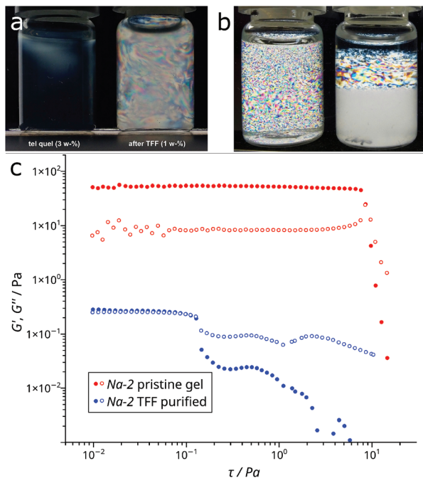
Fig. 7 (a) Birefringence of the crude gel of Na-2 (left vial) and of the TFF purified Na-2 (right vial). (b) Birefringence of the DMEA (left) and of the \text{NH}_3 (right) neutralized TFF purified dispersion of Na-2 (pH 8, aged for three months). (c) Amplitude sweeps (solid symbols = G' ) reveal the fluidity of the purified ribbons under shear. All dispersions comprised 1 weight-% ribbons, in contrast to the solid contents of the pristine gel (3 weight-%).
