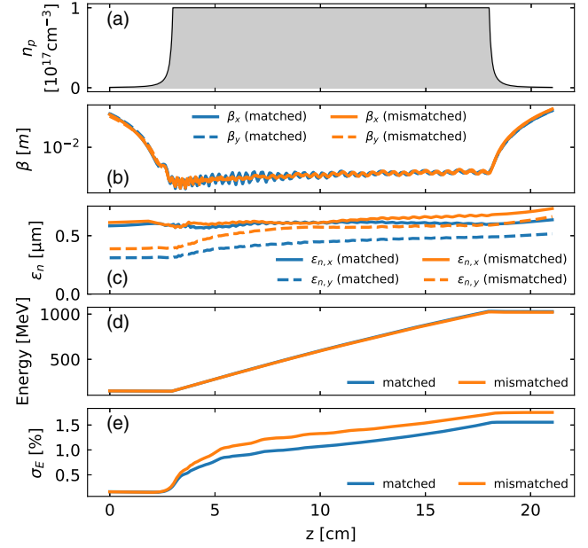
FIG. 8. Simulated evolution of beam parameters through an LPA plasma cell, using FBPIC code, in the ARES linac for the matched beam and the mismatched case 1 beam considered in this study.
