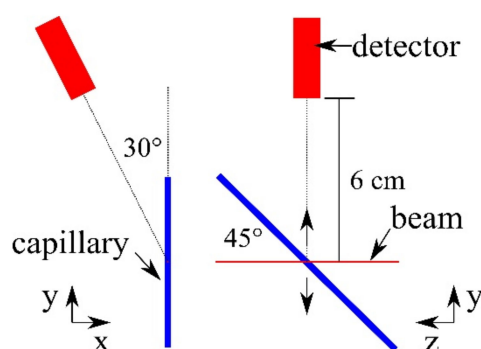
Figure 5. Schematic sketch of the capillary mount geometry. Left: frontal geometry, right: side view.
