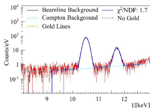
Figure 7. Capillary with agarose only, displaying two arsenic K_{\alpha} lines at 10.5 keV and two K_{\beta} at 11.72 keV, each fitted with a single Gaussian.
