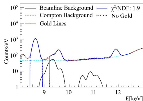
Figure 8. Cell mono layer showing zinc, below 9 keV and bromine above 12 keV.
