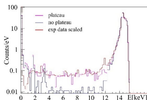
Figure 9. Comparison of simulated spectra with added plateau (magenta), no added plateau (blue), and an experimental spectrum (red).
