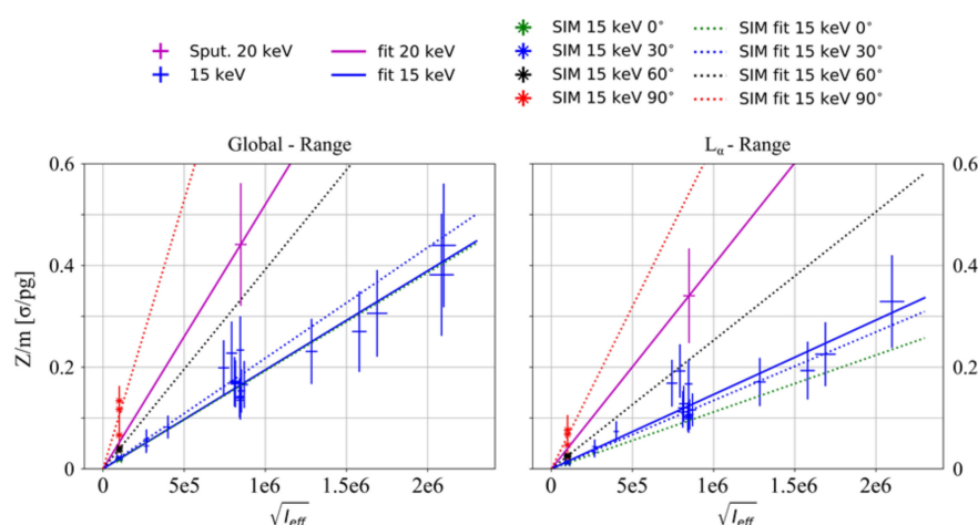
Figure 3. Significance [ \sigma ] per gold mass [pg] (i.e., total mass in beam-probe intersection) plotted over the root of effective incident photons for experimental and simulated data. Left: L_\alpha and L_\beta gold fluorescence regions were considered. Right: only L_\alpha on data is shown.
