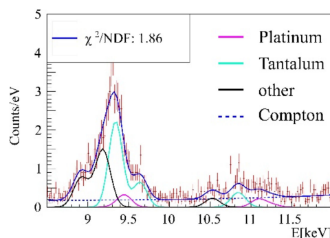
Figure 6. Background determination in the gold signal region, the main Ta (cyan) and Pt (pink) fluorescence lines are implemented accordingly to their intensities. Blue dotted: Compton background, black line: Other emission lines. Blue line: Fluorescence background for subsequent fits.
