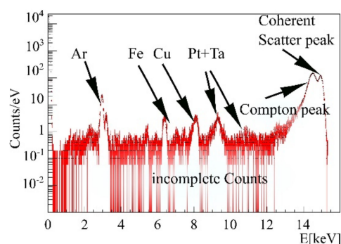
Figure 4. Measurement without sample. Beamline intrinsic fluorescence peaks are clearly visible.
