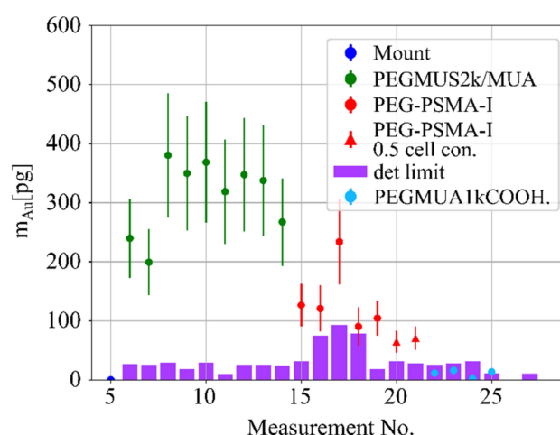
Figure 1. Reconstructed gold mass with corresponding detection limits (magenta) for four different probes, PEGMUA2k/MUA (green), PEG-PSMA-I (red dot), PEG-PSMA-I with half the number of cells in the beam (red triangle) and cells with PEGMUA1kCOOH nanoparticles (light blue dots). The nanoparticles were incubated at 12.5 nM with PC3 cells for 16 h, see Figure 2. The X-ray beam-sample-intersection volume, i.e., the volume of the sample which was interrogated by synchrotron radiation was 0.0889 mm 3 .
