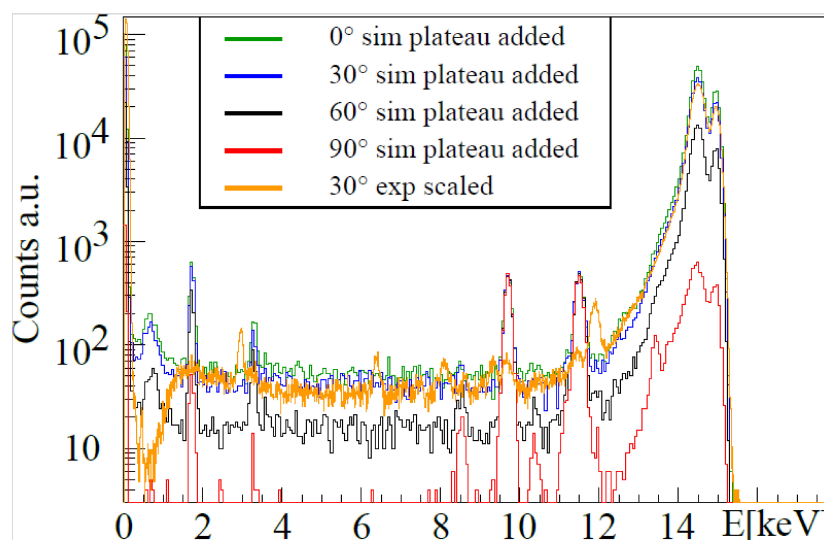
Figure 10. Simulated spectra with different detector angles, 0^\circ (green), 30^\circ (blue), 60^\circ (black), and 90^\circ (red). 90^\circ equals a detector placement in the plane of polarization. The Au concentration here was 0.01 mg/mL. The detector angle in the experimental case was 30^\circ for which an example spectrum is shown in yellow.
