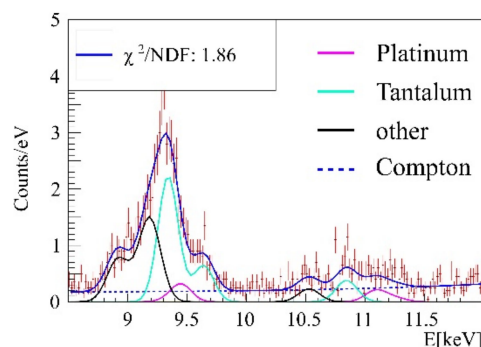
Figure 6. Background determination in the gold signal region, the main Ta (cyan) and Pt (pink) fluorescence lines are implemented accordingly to their intensities. Blue dotted: Compton background, black line: Other emission lines. Blue line: Fluorescence background for subsequent fits.
