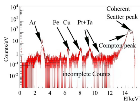
Figure 4. Measurement without sample. Beamline intrinsic fluorescence peaks are clearly visible.
