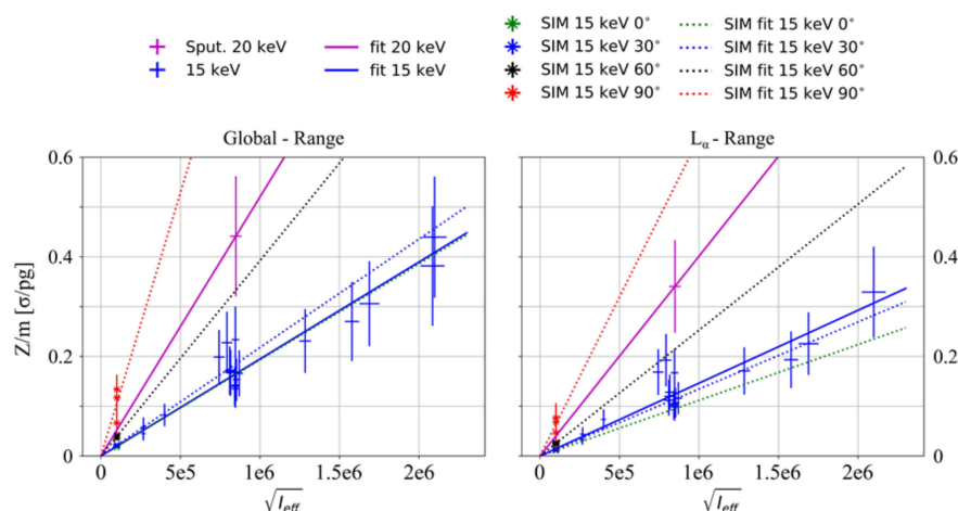
Figure 3. Significance [ \sigma ] per gold mass [pg] (i.e., total mass in beam-probe intersection) plotted over the root of effective incident photons for experimental and simulated data. Left: L_\alpha and L_\beta gold fluorescence regions were considered. Right: only L_\alpha on data is shown.
