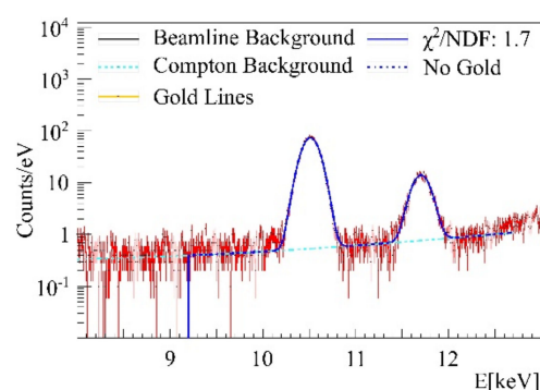
Figure 7. Capillary with agarose only, displaying two arsenic K_{\alpha} lines at 10.5 keV and two K_{\beta} at 11.72 keV, each fitted with a single Gaussian.
