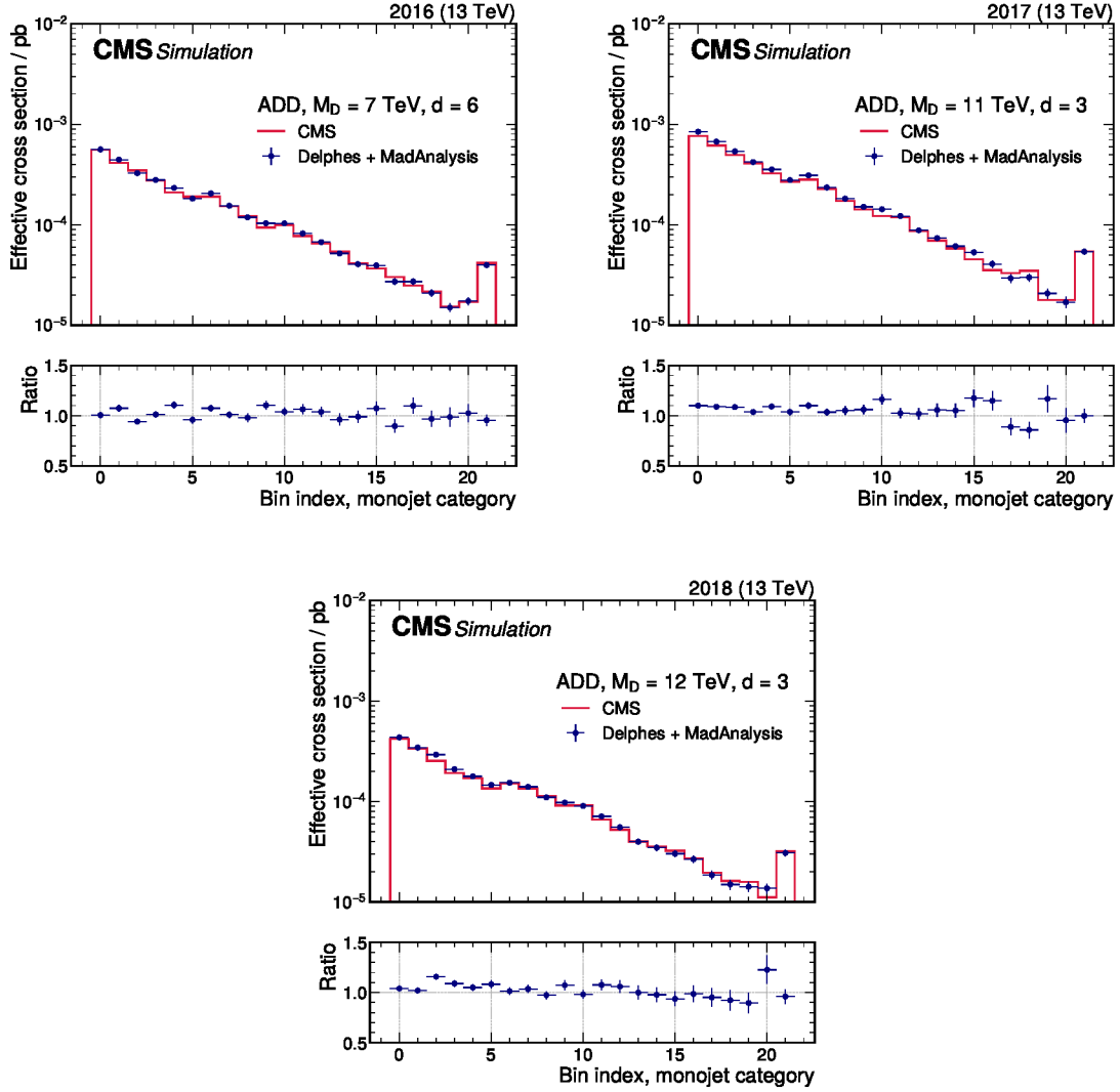
Figure 26. Comparison of the signal templates derived with DELPHES and MADANALYSIS (dark blue points) and the CMS analysis work flow (red solid line). The panels show three example parameter points for the ADD interpretation, and showcase the selection procedure for different years (2016 in the upper left, 2017 in the upper right, and 2018 in the lower panels). The rightmost bin includes the overflow. In all cases, the average agreement is observed to be better than 10%, with maximum deviations up to 20% in single bins.
