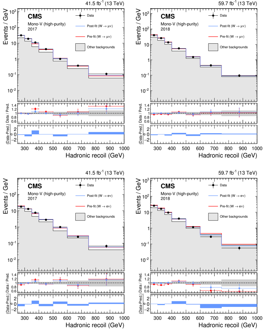
Figure 18. Hadronic recoil distributions in the single muon (upper), and single electron regions (lower) in the high-purity mono-V category. The “Other backgrounds” include top quark, diboson, and QCD multijet processes.
