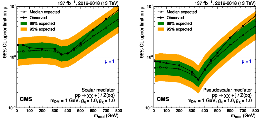
Figure 9. Upper limits at 95% CL on the signal strength \mu = \sigma/\sigma_{\text{theo}} as a function of m_{\text{med}} for scenarios with scalar (left) and pseudoscalar (right) mediators and coupling values of g_q = 1.0 , g_\chi = 1.0 , for a constant value of m_{\text{DM}} = 1 GeV. The blue solid line indicates the exclusion boundary \mu = 1 . In the case of a pseudoscalar mediator, m_{\text{med}} values up to 470 GeV are excluded (490 GeV expected).
