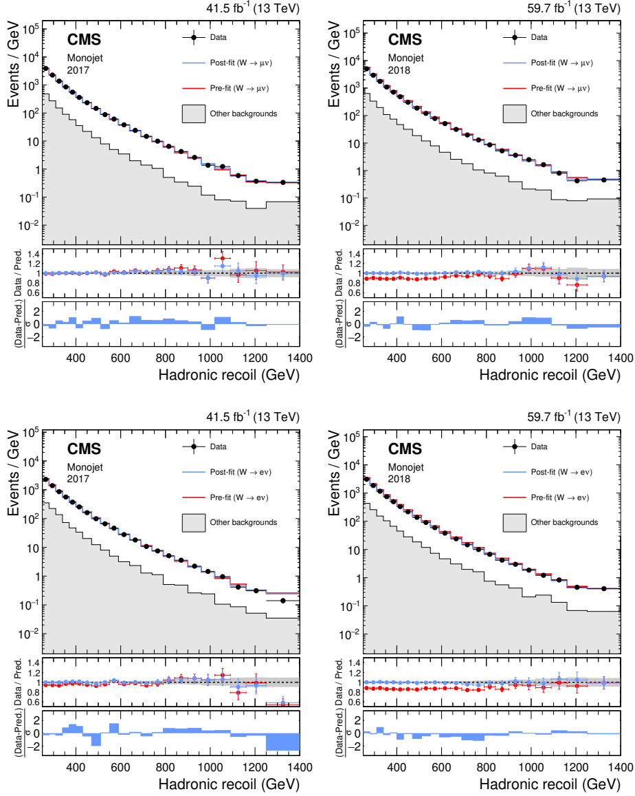
Figure 14. Hadronic recoil distributions in the single muon (upper), and single electron regions (lower) in the monojet category. The “Other backgrounds” include top quark, diboson, and QCD multijet processes.
