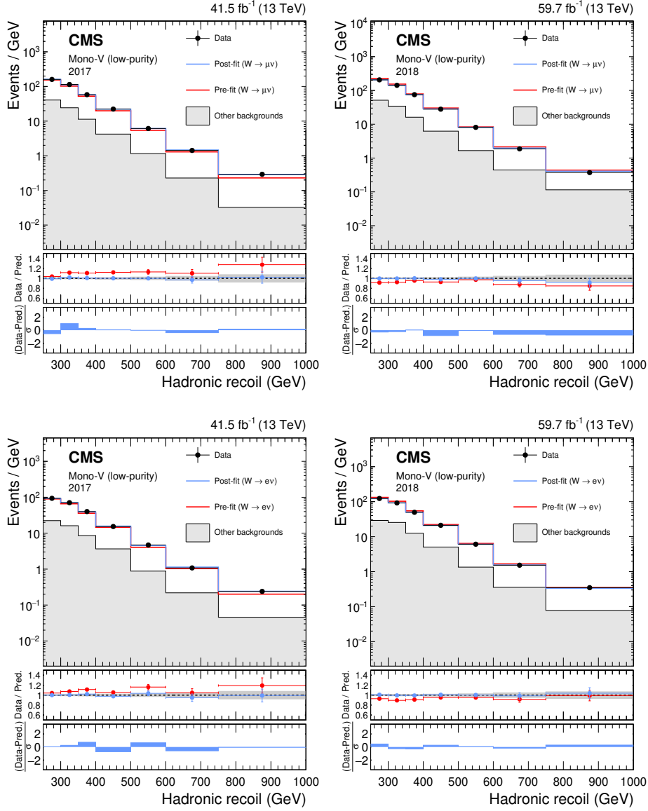
Figure 16. Hadronic recoil distributions in the single muon (upper), and single electron regions (lower) in the low-purity mono-V category. The “Other backgrounds” include top quark, diboson, and QCD multijet processes.
