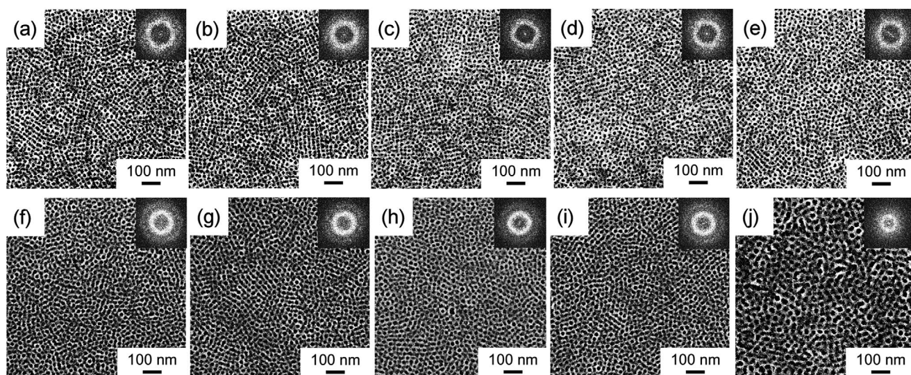
Figure 1. Top-view secondary electron SEM images of the \text{TiO}_2/\text{GeNC} films after thermal annealing at 500 °C in air: a) 0 wt%, b) 0.5 wt%, c) 1.0 wt%, d) 2.5 wt%, and e) 5.0 wt% GeNCs, or in argon atmosphere: f) 0 wt%, g) 0.5 wt%, h) 1.0 wt%, i) 2.5 wt%, and j) 5.0 wt% GeNCs. Insets show corresponding 2D-FFT patterns.
