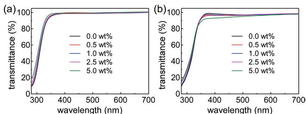
Figure 6. Transmittance spectra of the \text{TiO}_2/\text{GeNC} films containing indicated GeNC contents after thermal annealing in a) air and b) argon atmosphere. The glass substrate is used as a reference sample for the transmission measurement.
