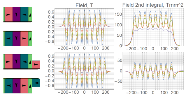
Figure 1: End field termination before (top) and after (bottom) modification, magnetic field and trajectory along beam direction [mm] for various gaps.
