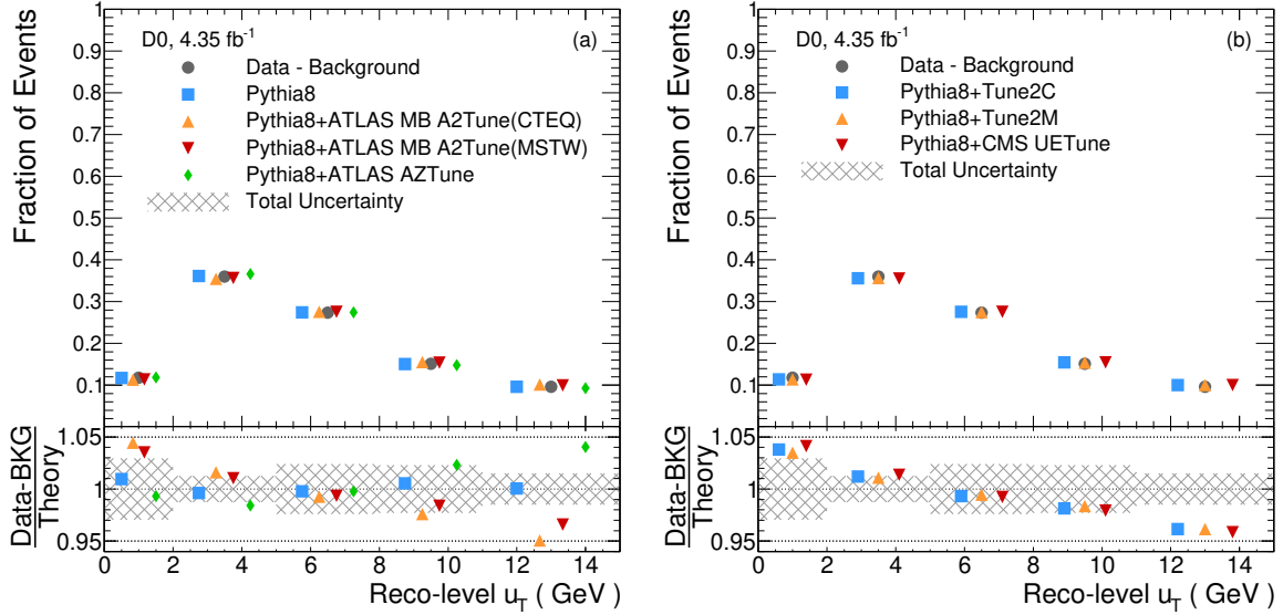
FIG. 4: [color online] Comparisons of the measured and predicted u_T distributions after the detector response simulation for different MC predictions based on PYTHIA. The ratios of the background-subtracted data to each theory prediction are shown in the lower panel together with the 1\sigma uncertainty band. The total experimental uncertainty is indicated by the hatched band; it is dominated by the uncertainty due to the hadronic recoil calibration. The points for the predictions are offset horizontally to aid with visibility.
