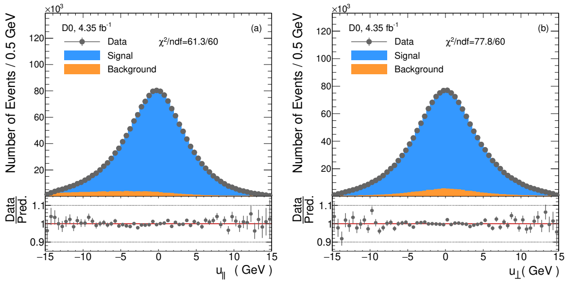
FIG. 2: [color online] Kinematic distributions for (a) u_{\parallel} , (b) u_{\perp} . The data are compared to the PMCS plus background prediction in the upper panel, and the ratio of the data to the PMCS plus background prediction is shown in the lower panels. Only the statistical uncertainty is included.
