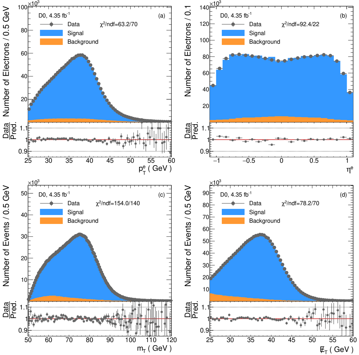
FIG. 1: [color online] Kinematic distributions for (a) p_T^e , (b) \eta^e , (c) m_T , (d) E_T . The data are compared to the PMCS plus background prediction in the upper panel, and the ratio of the data to the PMCS plus background prediction is shown in the lower panels. Only the statistical uncertainty is included.
