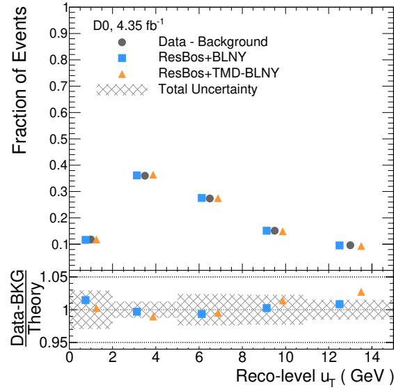
FIG. 3: [color online] Comparisons of the measured and predicted u_T distributions after the detector response simulation for different MC predictions based on RESBOS. The ratios of the background-subtracted data to each theory prediction are shown in the lower panel together with the 1\sigma uncertainty band. The total experimental uncertainty is indicated by the hatched band; it is dominated by the uncertainty due to the hadronic recoil calibration. The points for the predictions are offset horizontally to aid with visibility.
