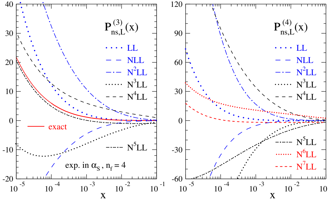
Figure 1. Successive small- x approximations to the N^n LO four-flavour splitting functions P_{ns,L}^{(n)}(x) in the large- n_c limit for n = 3 (left), compared to the exact result, and n = 4 (right). The respective N^5LL and N^7LL curves include all terms with x^0 \ln^k x at k > 0 as specified by eqs. (3.3), (3.4) and (3.8)–(3.15).
