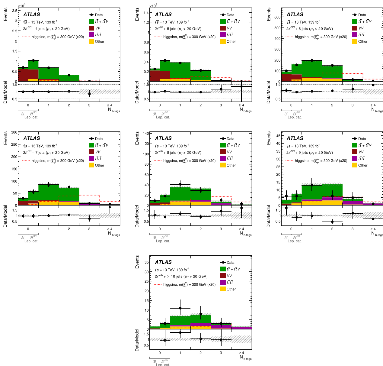
Fig. 6 The observed data event yields and the corresponding estimates for the backgrounds in the different b -jet multiplicity bins for the 20 GeV \text{jet-}p_T threshold regions defined for the EWK analysis in the 2\ell^{SC} category. The background shown is estimated by including all bins in the fit.
