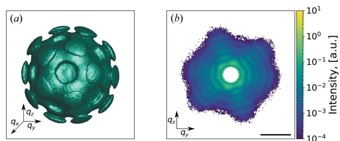
Figure 6 Reciprocal space representation for the MaxF1 selection with the EM algorithm and size filtering applied. (a) 3D intensity distribution of the virus in reciprocal space after background subtraction. (b) 2D cut of the distribution. All diffraction patterns are shown in logarithmic scale. The black scale bar denotes 0.5 \text{ nm}^{-1} .
