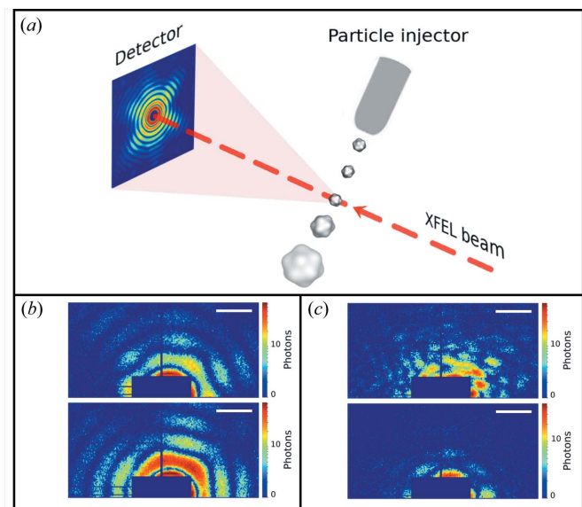
Figure 2 (a) Schematic representation of an SPI experiment. The incoming XFEL beam interacts with the virus injected by the particle injector. The particle is destroyed afterwards owing to Coulomb explosion. X-ray radiation from the non-destroyed virus is scattered to the detector positioned in the far field. (b) Examples of single hits. (c) Examples of non-single hits. The diffraction patterns in (b) and (c) are shown in logarithmic scale; an area of size 192 \times 96 pixels from the whole diffraction pattern is shown. The scale bars in (b) and (c) correspond to 0.2 \text{ nm}^{-1} .
