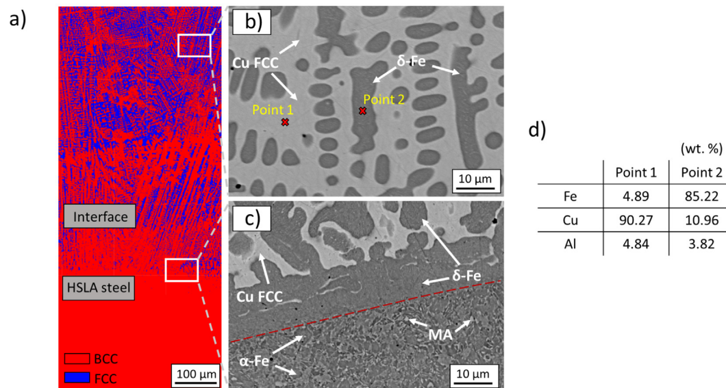
Fig. 8. (a) EBSD phase mapping of the interface region; (b) SEM morphologies of \delta -ferrite in a Cu FCC matrix; (c) SEM morphologies of MA constituents in an \alpha -Fe matrix; (d) EDS point analysis at positions marked in (b). MA: Martensite-austenite.
