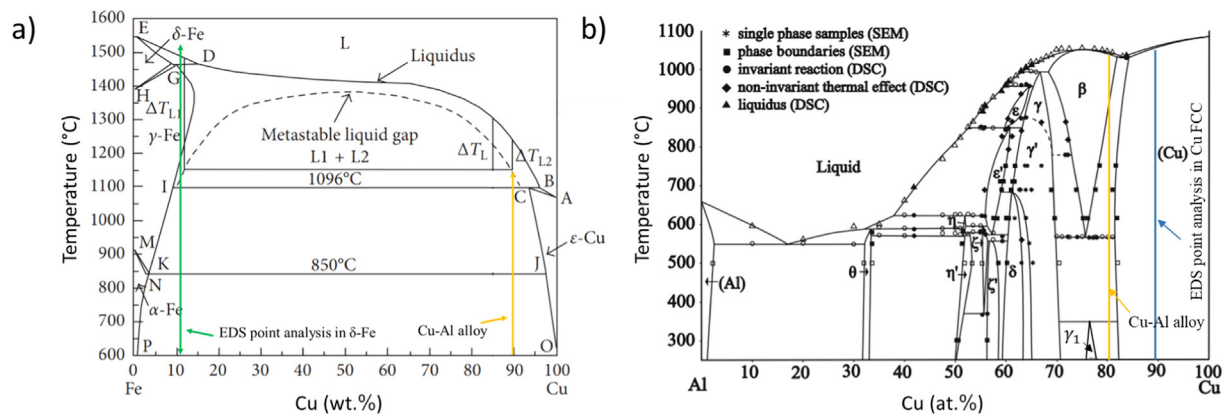
Fig. 12. (a) Cu–Fe Phase diagram with the metastable miscibility gap (dotted curved line) (adapted from [27]), pointing to the composition of the δ-Fe constituent; (b) Cu–Al binary phase diagram highlighting the composition in the Cu-FCC constituents in the interface (adapted from [28]).
