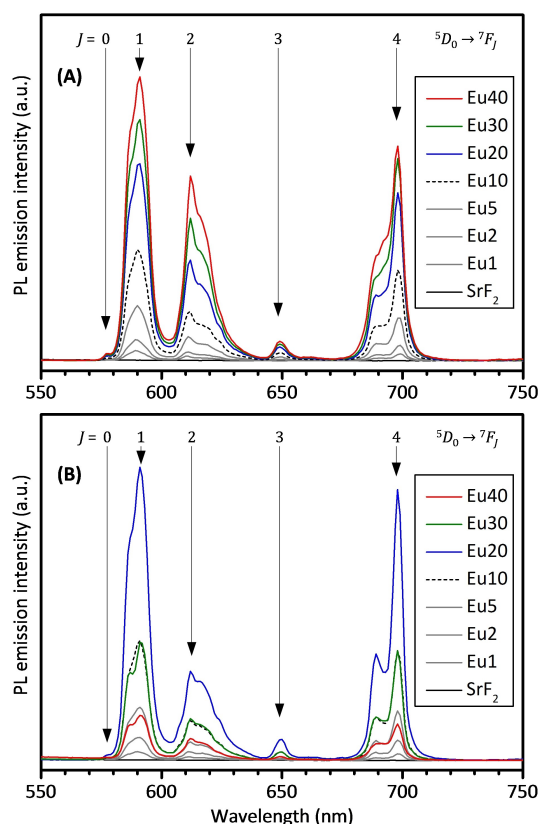
Figure 3. PL emission spectra of 0.3 M sols of \text{Sr}_{1-x}\text{Eu}_x\text{F}_{2+x} in ethylene glycol ( \lambda_{\text{ex}} = 393 nm). (A) as-synthesized, (B) annealed at 160^\circ\text{C} .
