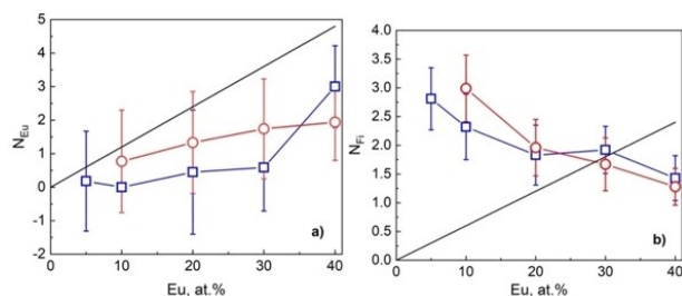
Figure 11. Sr coordination number for Sr...Eu pairs (a) and Sr...F i pairs (b) according to Sr-K EXAFS spectra. Bold lines show regular distribution; □ correspond to as synthesized samples; ○ correspond to heat-treated samples.
