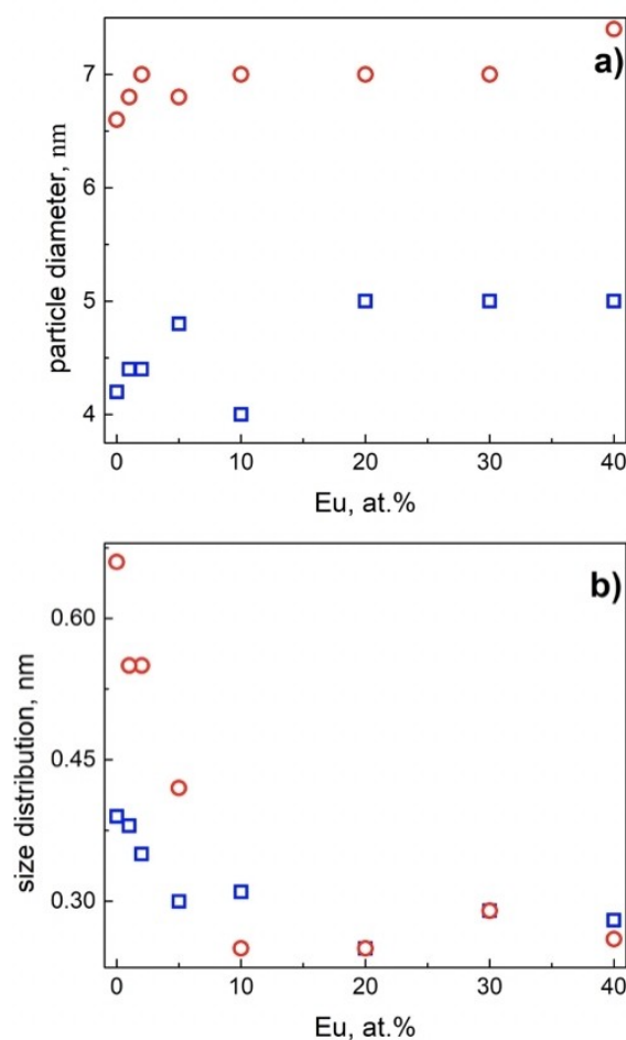
Figure 7. Average particle diameter ( D = 2Ra , a) and particle size distribution ( sig , b) for as synthesized (□) and annealed (○) \text{Sr}_{1-x}\text{Eu}_x\text{F}_{2+x} samples obtained using small-angle X-ray scattering (according to Table 2).
