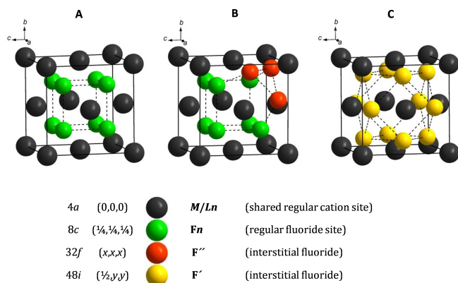
Figure 2. Fluoride clusters found in solid solutions \text{MF}_2\text{-LnF}_3 ( \text{M}_{1-x}\text{Ln}_x\text{F}_{2+x} ; x=0\text{--}\approx 0.45 ; \text{M}=\text{Ca}, \text{Sr} ; \text{Ln}=\text{Y}, \text{La-Lu} ). Wyckoff symbols are for space group \text{Fm}\bar{3}\text{m} (225). (A) Undisturbed fluorite structure of \text{MF}_2 ( x=0 ). (B) Triangular cluster defects for 32 f positions ( x \geq 0.01 ). (C) Cubeoctahedral cluster defects for 48 i positions ( x \geq 0.01 ). [13–15]
