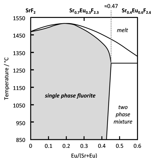
Figure 1. Sr-rich part of the equilibrium phase diagram \text{SrF}_2\text{-EuF}_3 . Phase diagrams of all combinations \text{MF}_2\text{-LnF}_3 ( M = \text{Ca, Sr} ; \text{Ln} = \text{Y, La-Lu} ) are qualitatively similar. [3]
