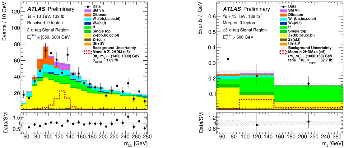
(a) Invariant di- b -jet mass distribution for the 2 b -tag, 350 \text{ GeV} < E_T^{\text{miss}} < 500 \text{ GeV} region.
