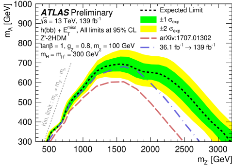
(a) Parameter convention used in the previous iteration ( m_H = m_{H^\pm} = 300 GeV).
