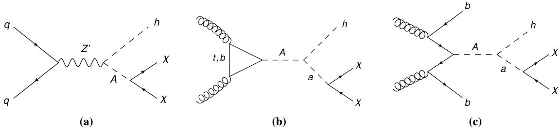
Figure 1: Dominant Feynman diagrams for the mono-Higgs signature production using the Z' -2HDM (a) and the 2HDM+a (b, c) models.
