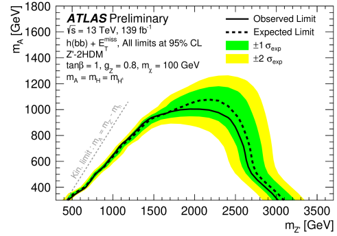
(b) New parameter convention ( m_H = m_{H^\pm} = m_A ).
