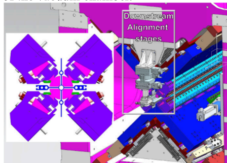
Figure 2: Layout of the alignment stages and a cross-section of the vacuum chamber surrounded by four magnetic structures at the minimum gap.
