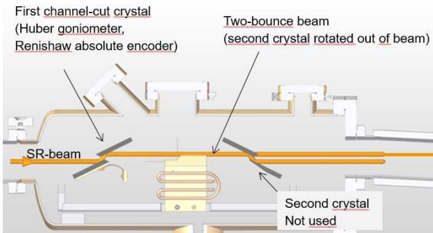
Figure 3: Schematic of the K-Mono. The monochromator is placed about 160 m behind the undulator section. For these measurements we use the “two bounce” beam which hits a GOS screen and is observed by the imager with a 14.3 \mu\text{m} pixel size.
