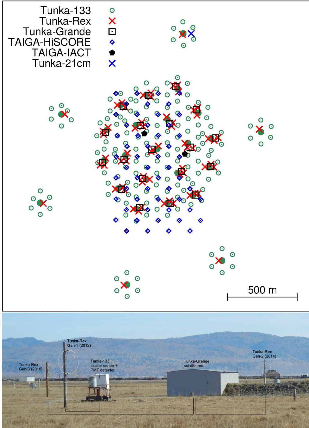
Figure 1: The layout of the TAIGA setups as of 2019. The antenna stations are depicted as crosses (the Tunka-21cm array is depicted by a single marker due to scale of the map). The layout and hardware configuration was changes several times during the past years. Bottom: Photo of a single cosmic-ray cluster of the TAIGA facility. Lines mark the cable connections.
