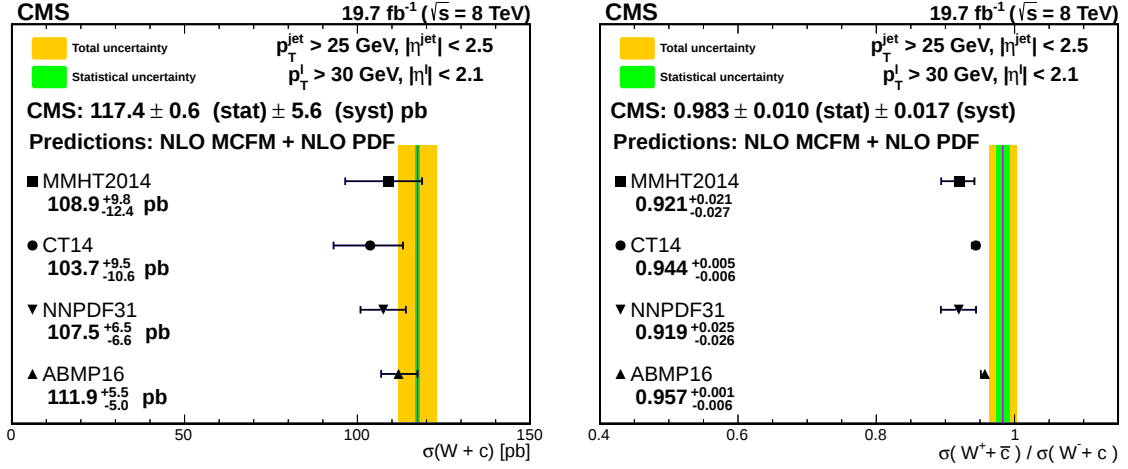
Figure 4: Comparison of the theoretical predictions for \sigma(W+c) (left) and \sigma(W^++\bar{c})/\sigma(W^-+c) (right) computed with MCFM and several sets of PDFs with the current experimental measurements.
