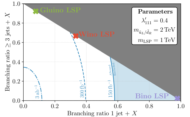
FIG. 2. Projected constraints based on integrated luminosities of (150, 300, 3000) \text{ fb}^{-1} shown as blue-(solid, dashed, dot-dashed) contours. These constraints are shown as a function of the branching ratios into the two channels: (i) 1 \text{ jet} + X , (ii) \geq 3 \text{ jets} + X where X denotes either an electron or a neutrino. As reference points, we show the expected branching ratios for an RPV model featuring a 1 TeV gluino, bino or wino-LSP, see Section IV A for more details.
