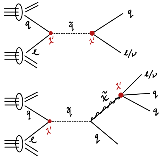
FIG. 1. Resonant squark produced via the \lambda'_{ijk} L_i Q_j \bar{D}_k operator at the LHC followed by its direct decay mode (top) and decay via an example of a gauge-cascade mode (bottom). Here \tilde{\chi} denotes a chargino or neutralino, lighter than the squark.
