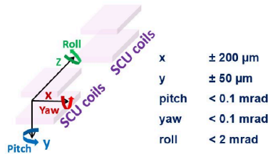
Figure 4: Sketch of the two SCU coils with the reference axes and angles, and the maximum allowed misalignment between them.
