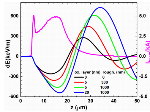
Figure 5: Current profile of the electron bunch for a charge of 250 pC (magenta line). Energy change per meter for a copper pipe with 5 mm diameter and a surface, without oxide layer and roughness (black line), with an oxide layer of 5 nm and 300 nm roughness (red line), with an oxide layer of 5 nm and 1000 nm roughness (green line), and with an oxide layer of 20 nm and 1000 nm roughness (blue line).
