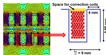
Figure 3: Left: FEMM simulations of the 18 mm period SCU coils. The magnetic flux lines are indicated. The color scales with the absolute value of the magnetic flux density (magenta highest to cyan). Right: Geometry of the SCU coils: the red circles represent the wire in the groove.
