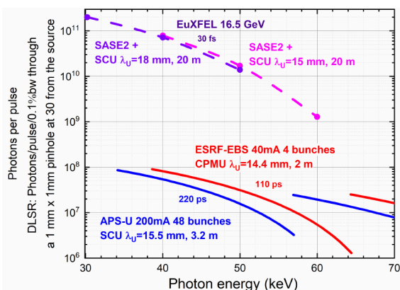
Figure 2: Photons per pulse generated by the afterburner, made of five SCU modules with both 15 and 18 mm period length and a magnetic length of 20 m, are shown as a function of the photon beam energy. The calculation has been done using the code GENESIS 1.3 v.2 [2], with the electron beam parameters shown in Table 1. The photons per pulse are compared to the ones calculated using SPECTRA [3] from typical short period undulators at the ESRF-EBS [4] and APS-U [5] through a pinhole of 1 \text{ mm} \times 1 \text{ mm} at 30 m from the source.
