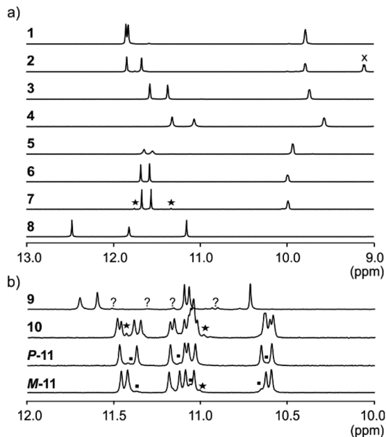
Fig. 3 Excerpts from the 500 MHz ^1\text{H} NMR spectra of (a) compounds 1–8 recorded at 25 °C in \text{H}_2\text{O}/\text{CD}_3\text{CN} 75 : 25 (v/v) and (b) compounds 9 and 10, 11 recorded at 25 °C in \text{H}_2\text{O}/\text{D}_2\text{O} 9 : 1 (v/v), and \text{H}_2\text{O}/\text{CD}_3\text{CN} 1 : 1 (v/v), respectively. The spectra show amide resonances i.e. typically all NHs belonging to Q and some NHs belong to P units. Other NHs belonging to P units are found at lower field and overlap with aromatic resonances. X indicates the signal of an aromatic proton. Resonances marked with stars have been interpreted as impurities. Squares in the spectra of P -11 and M -11 correspond to the other diastereoisomer resulting from incomplete separation. Resonances marked with (?) in 9 could be an impurity or the other diastereomeric conformer.
