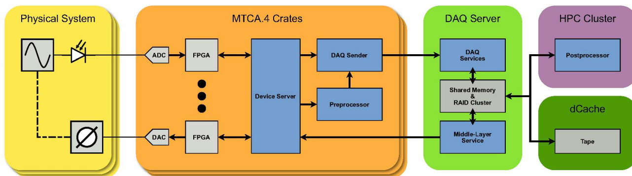
Figure 1: Data acquisition flow overview.
