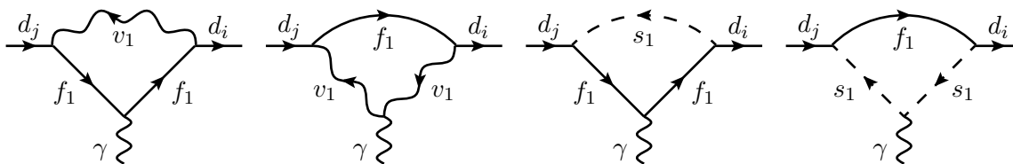
Figure 1. Diagrams for the off-shell d_j \rightarrow d_i \gamma Green’s function. Physical scalars are denoted by dashed lines, while the contribution of massive vector bosons and their related Goldstone bosons are denoted by a wavy line.
