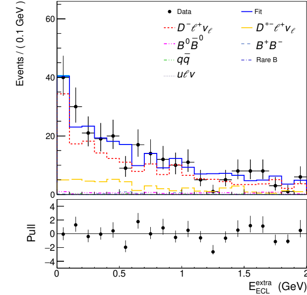
FIG. 1. Fit results for M_{\text{miss}}^2 (upper) and E_{\text{ECL}}^{\text{extra}} (lower) for the decays B^0 \rightarrow D^{(*)} \ell^+ \nu_\ell . The dots with error bars represent the data, and the blue line indicates the fitted results with the cyan band for fit uncertainty. The dashed lines indicate different fit components. E_{\text{ECL}}^{\text{extra}} is plotted with the selection M_{\text{miss}}^2 < 0.5 \text{ GeV}^2/c^4 .
