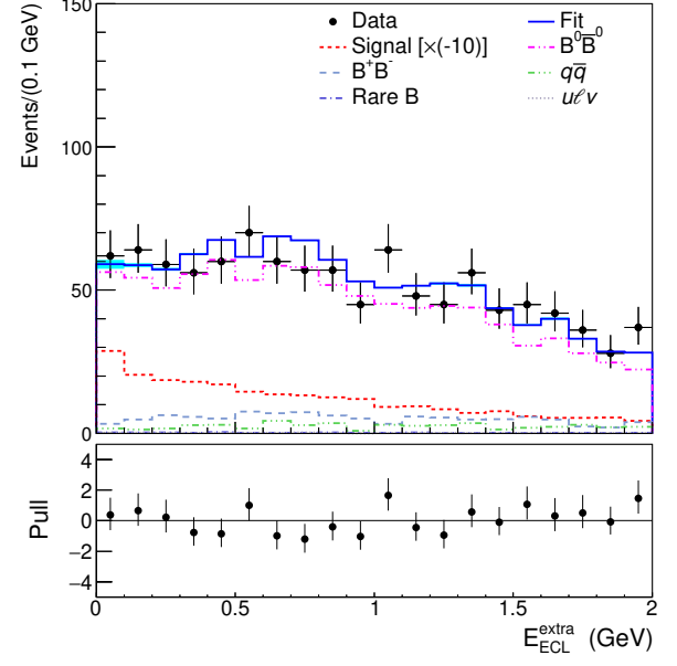
FIG. 2. Distribution of E_{\text{ECL}}^{\text{extra}} combined for all signal modes. The dots with error bars show the data, the blue line shows the fitted results with the cyan band for fit uncertainty, and the dashed lines show fit results for the different components. The signal component is scaled with a factor of -10.
