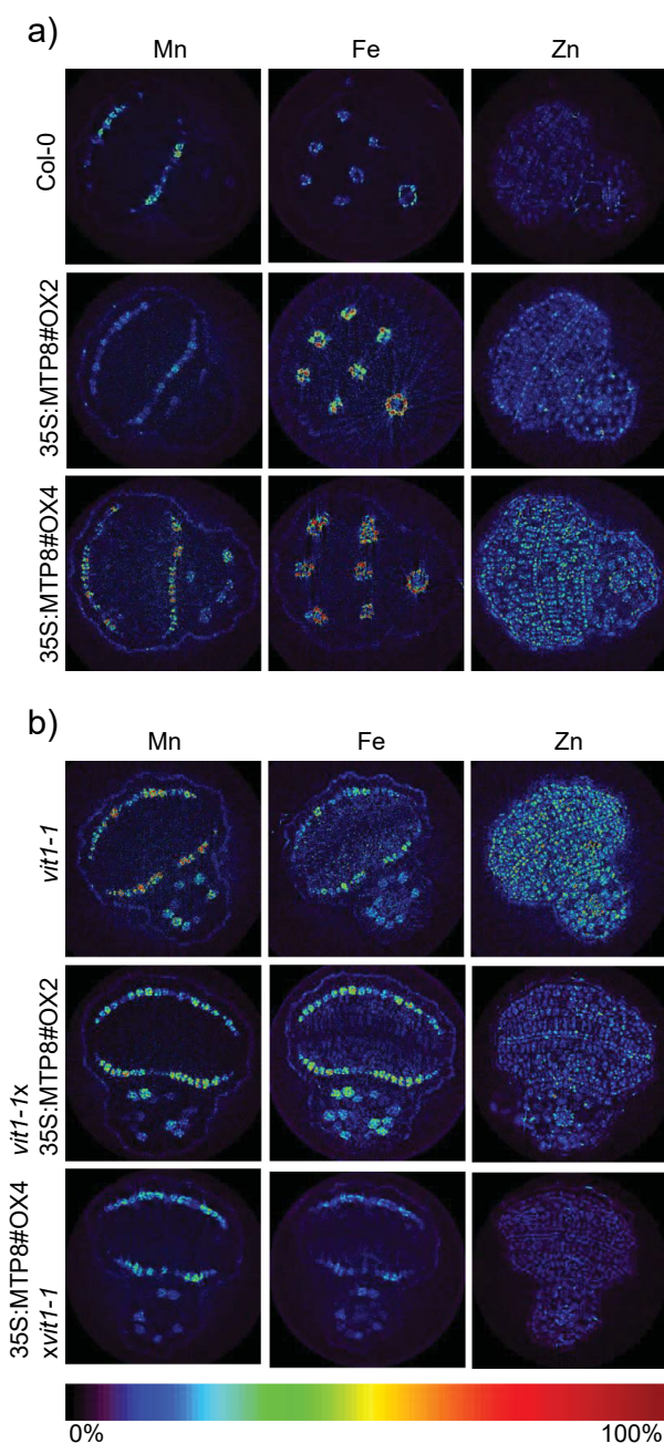
Fig. 4. Metal distribution in A. thaliana seeds; (a) Col-0 and 35S:MTP8 lines; (b) vit1-1 and 35S:MTP8x vit1-1 lines. \mu XRF tomographs of intact seeds showing the distribution of Fe, Mn and Zn. The colour scale ranges from 0 to 500 \mu\text{g}\cdot\text{g}^{-1} for all metals.
