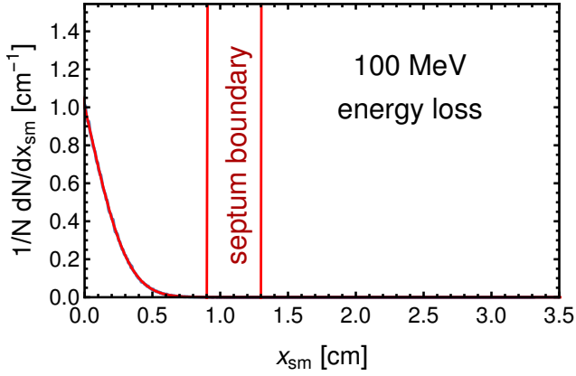
Fig. 7 Transverse coordinate distribution of the beam at the position of the septum magnet with the condition of a constant angular kick of the deflection device of 1.75 mrad, taking into account the energy loss in the deflection device of 100 MeV. The vertical lines indicate the septum magnet boundary. The red curve indicates the result of a Gaussian fit
