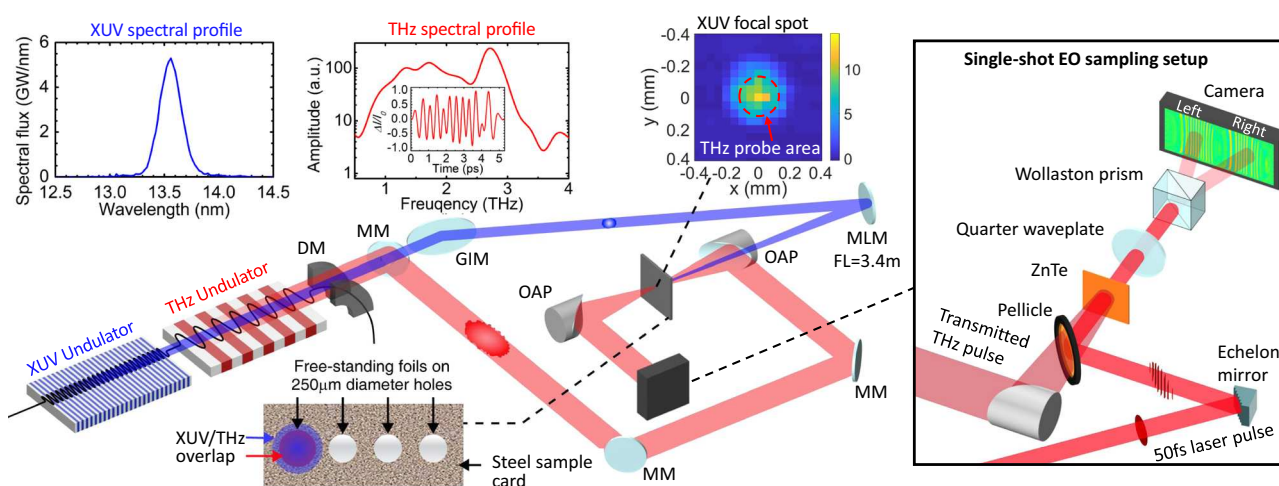
Fig. 1 The experimental setup to measure terahertz (THz) transmission through free-standing gold foils excited by extreme ultraviolet (XUV) pulses.
