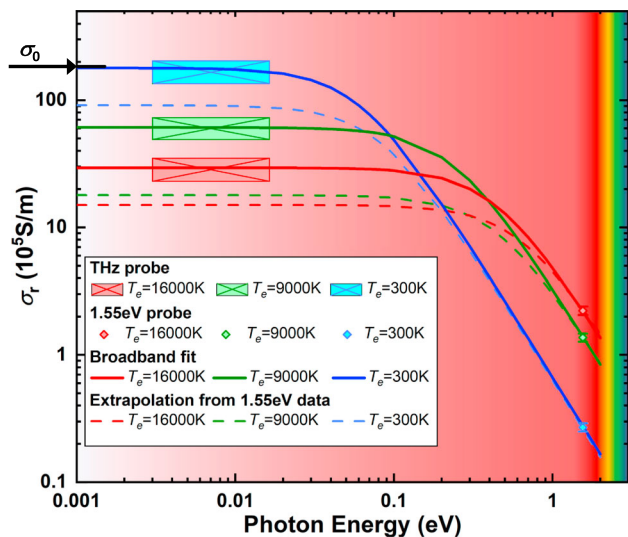
Fig. 3 The electrical conductivity as a function of photon energy for various excitation conditions of solid gold. The broadband electrical conductivity data (real part, \sigma_r ) at electron temperatures of T_e = 300 K (blue), 9000 \pm 900 K (green) and 16,000 \pm 1500 K (red) are indicated by the different colors; the THz conductivity at small photon energies (0.75–3.75 THz in frequency, or 3–15.5 meV in photon energy) are shown as square blocks that cover the range of frequency components in the THz cycles (horizontal dimension) and uncertainties of the inferred conductivity values (vertical dimension), the optical conductivity at higher photon energies (1.55 eV) from ref. 30 are presented as diamonds, and the DC conductivity at room temperature measured with four-point probe is pointed out by a black arrow. The solid curves represent the Drude model fit through the high and low frequency data, and the dashed curves represent Drude model extrapolation from the optical conductivity values at 1.55 eV using the Drude model. The conductivity measured with THz radiation agrees well with the DC conductivity from four-point probe measurements, while the extrapolation from optical measurements shows significant discrepancies.
