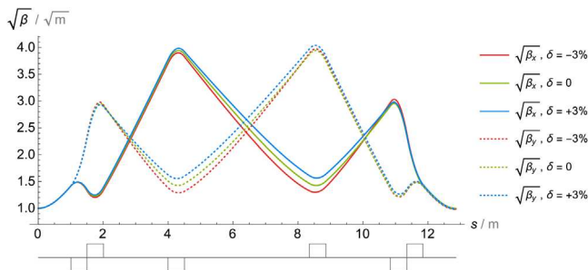
FIG. 12. Illustration of apochromatic correction in a lattice of only linear focusing optics (six quadrupole magnets). The lattice is constructed such that beta functions evolve differently for the various energy slices but eventually converge before entering the next stage. This method also works for plasma lenses and plasma density ramps. Source: Ref. [40] (CC BY 3.0).
