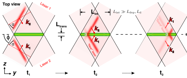
FIG. 15. Illustration of the traveling-wave electron acceleration scheme: Two lasers are coupled in transversely into an on-axis plasma channel. The superposition of the two lasers drives a wakefield, and, since the laser pulse fronts are tilted, the traveling wave can be made to move at speed c . Source: Ref. [125] (CC BY 4.0).
