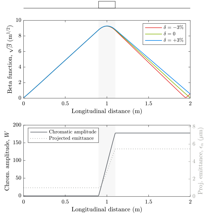
FIG. 3. Example of emittance growth due to chromaticity. A 10 GeV beam with 3% rms energy spread diverges from a plasma accelerator of density 10^{16} \text{ cm}^{-3} ( \beta_m \approx 10 \text{ mm} ). A simple beam optics lens captures and refocuses the beam into the next stage, which introduces significant chromaticity. As a result, the projected (energy-averaged) emittance increases by more than a factor of 5.
