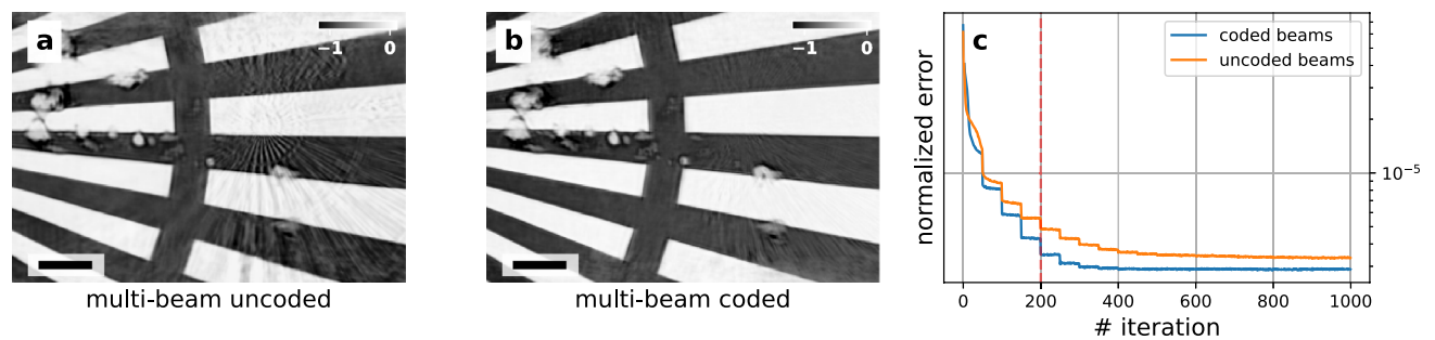
Figure 3. Cropped intermediate reconstruction results of the Siemens star after 200 iterations using (a) similar probes and (b) coded probes. The scale bars have a length of 1.5 μm. The grayscale indicates phase shift in radians. (c) Comparison of the evolution of the normalized error during the reconstruction of the scan of the Siemens star test sample with uncoded beams and coded beams. The sharp downward steps every 50 iterations are a result of the position correction being performed at these iterations.
