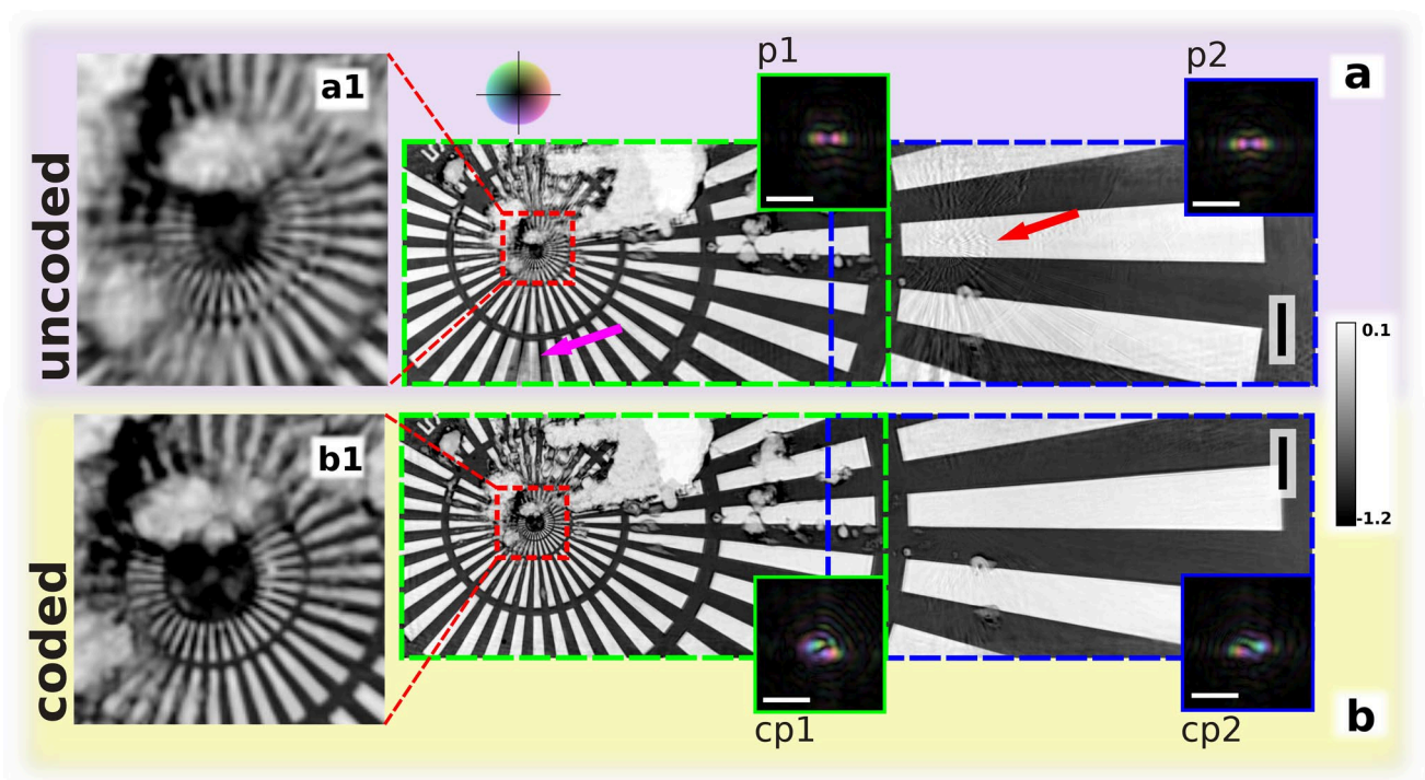
Figure 2. Reconstructed images of a Siemens star test sample and corresponding probes. Red and purple arrows show reconstruction defects. Blue/green dashed rectangles show which probe scanned which region of the sample: (a) uncoded probe case with the probes shown in (p1) and (p2), (a1) is the magnified center of the test pattern; (b) coded probe case, with the probes shown in (cp1) and (cp2), (b1) is the magnified center of the test pattern. The vertical scale bars represent 3 \mu\text{m} , the horizontal scale bars represent 4 \mu\text{m} . The gray scale indicates the sample phase shift in radians. Phases of the probes are color-coded.
