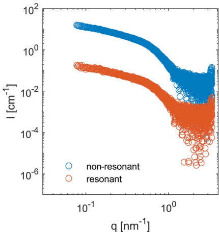
Figure 5 The resonant and non-resonant terms for ferritin calculated using equation (10).
