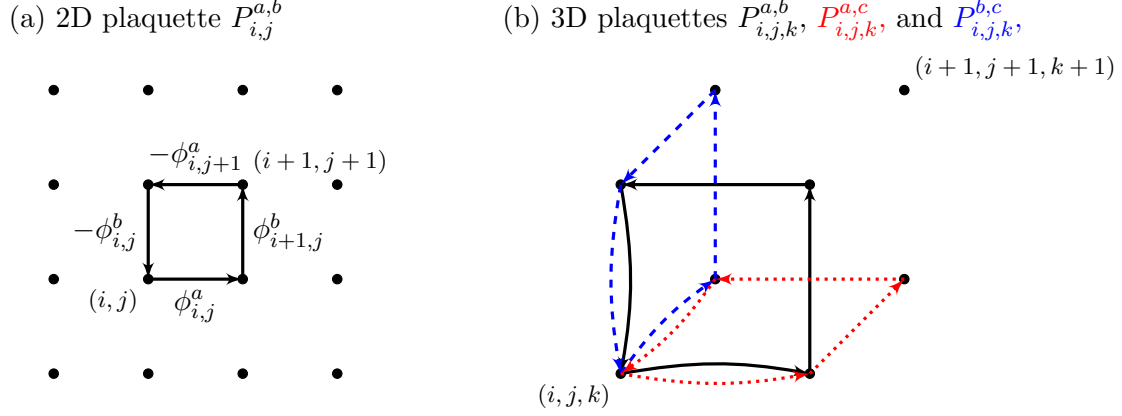
Figure 2: Construction of the plaquette in two (left) and three (right) dimensions. In two dimensions, the plaquette P_{i,j}^{a,b} at lattice point (i,j) is constructed by transporting the field along the path (i,j) \rightarrow (i+1,j) \rightarrow (i+1,j+1) \rightarrow (i,j+1) \rightarrow (i,j) . The field transformation along this path is given by (17). The angles \phi contribute with a positive sign if moving right or up, and with a negative sign if moving left or down. Left/right movement is labeled with a superscript a and up/down movement with superscript b . In three dimensions an additional forward/backward movement is denoted by the superscript c . Furthermore, there are three independent smallest loops that can be taken; namely in the (a,b) -plane (black solid line), (a,c) -plane (red dotted line), and (b,c) -plane (blue dashed line). Each of these planes equally contribute a “2-dimensional” plaquette. We note that all links are straight lines which we have bent simply for better visualization.
