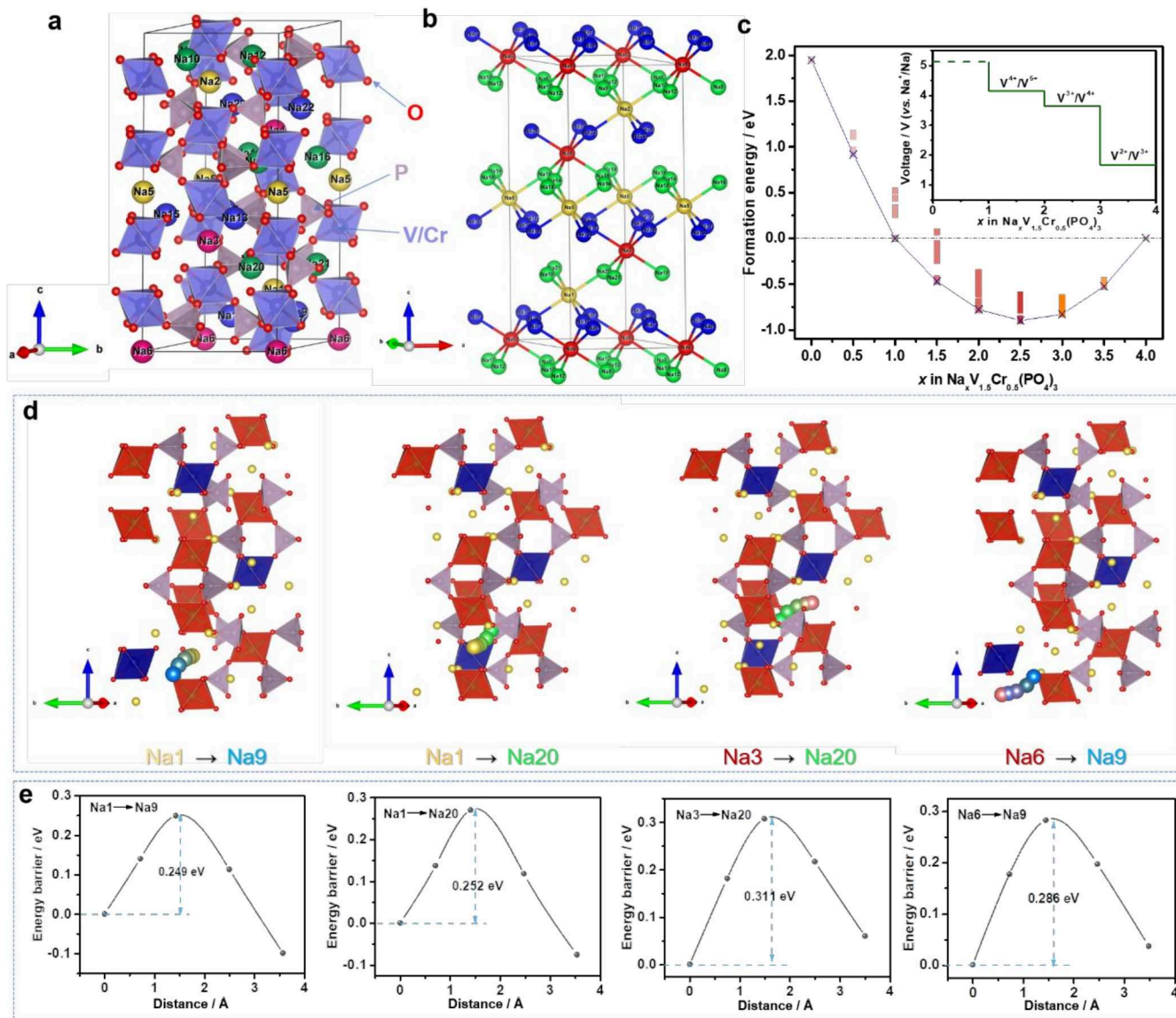
Figure 5 DFT calculation results of possible \text{Na}^+ ion diffusion pathways, and the corresponding migration energy barriers and formation energies in a single unit cell. (a) Illustration of the crystal structure of \text{Na}_3\text{V}_{1.5}\text{Cr}_{0.5}(\text{PO}_4)_3 with four different types of Na ions. (b) All of the four types of Na ions in a unit cell. (c) Formation energy (convex hull) of \text{Na}_x\text{V}_{1.5}\text{Cr}_{0.5}(\text{PO}_4)_3 ( x = 0, 0.5, 1, 1.5, 2, 2.5, 3, 3.5 and 4 ) from the DFT study. The inset is the calculated voltage profiles for \text{Na}_x\text{V}_{1.5}\text{Cr}_{0.5}(\text{PO}_4)_3 ( x = 0, 1, 2, 3 , and 4 ). (d) Calculated \text{Na}^+ ion diffusion pathways of the A-to-B type (Na1 to Na9), A-to-C type (Na1 to Na20), D-to-C type (Na3 to Na20) and the D-to-B type (Na6 to Na9). (e) Corresponding migration energy barriers within the different \text{Na}^+ ion groups as illustrated in (d).
