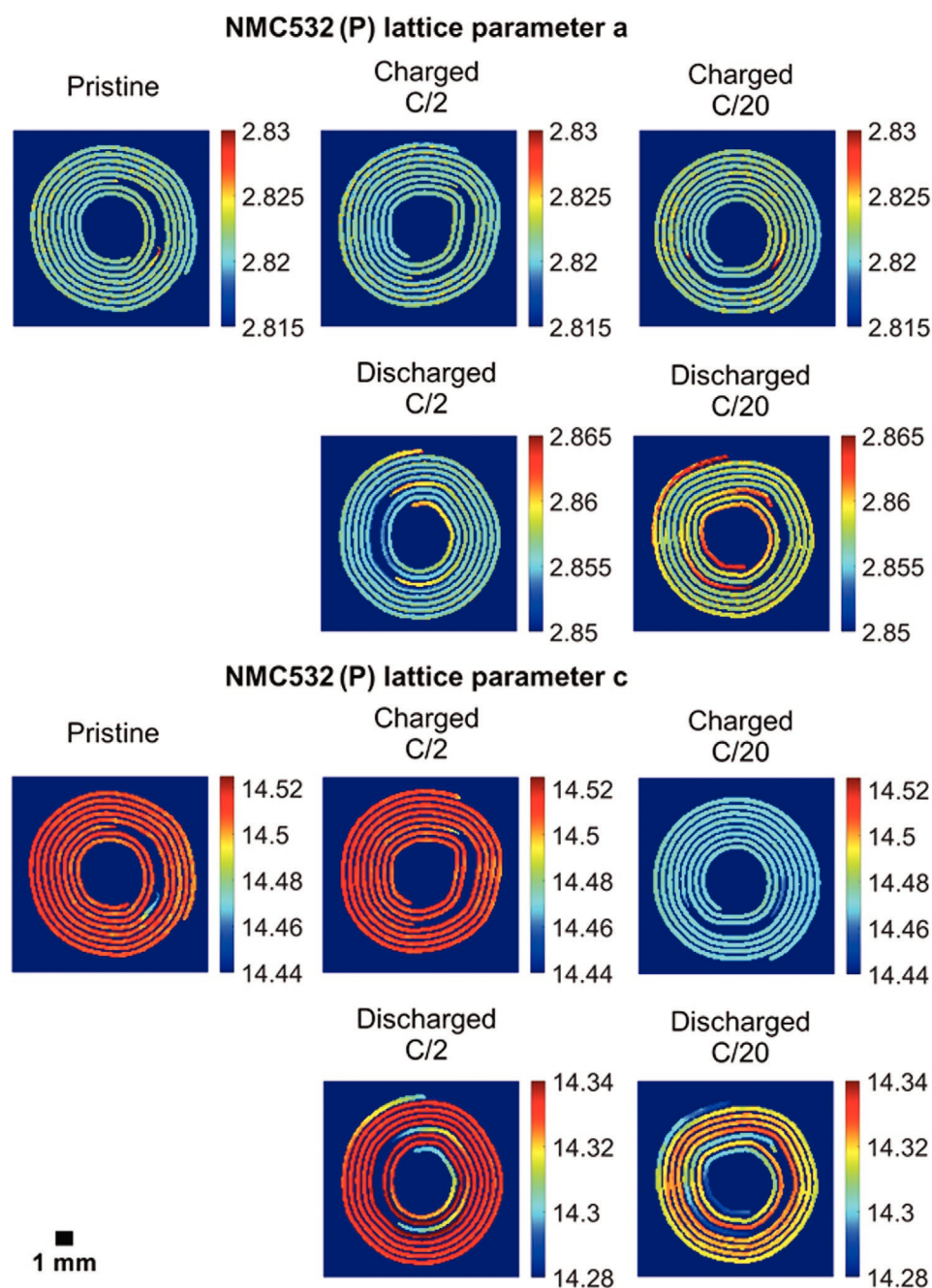
Figure 6. Lattice parameter a (top panel) and c maps (bottom panel) for the primary hexagonal NMC532 phase obtained with the DLSR algorithm. Colorbar units correspond to Å.
