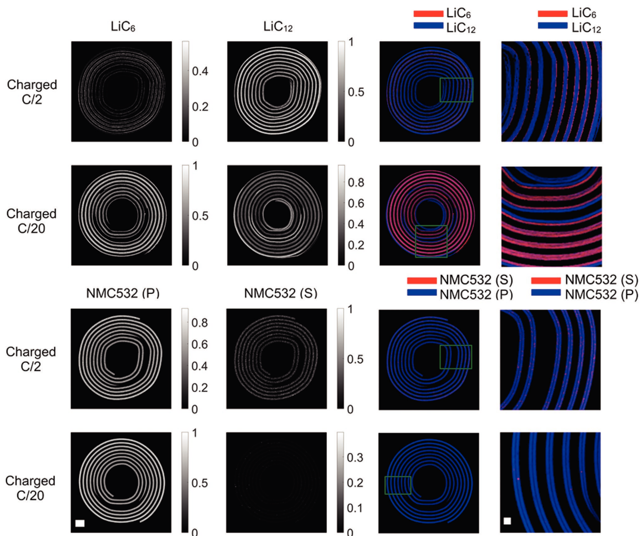
Figure 5. Phase distribution maps of the crystalline phases present in the anode (top panel) and in the cathode (bottom panel) of two charged cells with different cycling rates (C/2 and C/20). Scale bar in the bottom left corresponds to 1 mm (all electrode maps) and in the bottom right to 0.2 mm (magnified electrode map).
