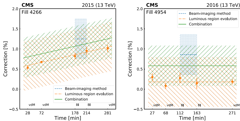
Fig. 14 Ratio of the \sigma_{\text{vis}} evaluated from the overlap integral of the reconstructed single-bunch profiles in two (BI method) or three (luminous region evolution) spatial dimensions to that determined by the vdM method, assuming factorization, and their combination. The central values are displayed as points or with a line while the corresponding full
