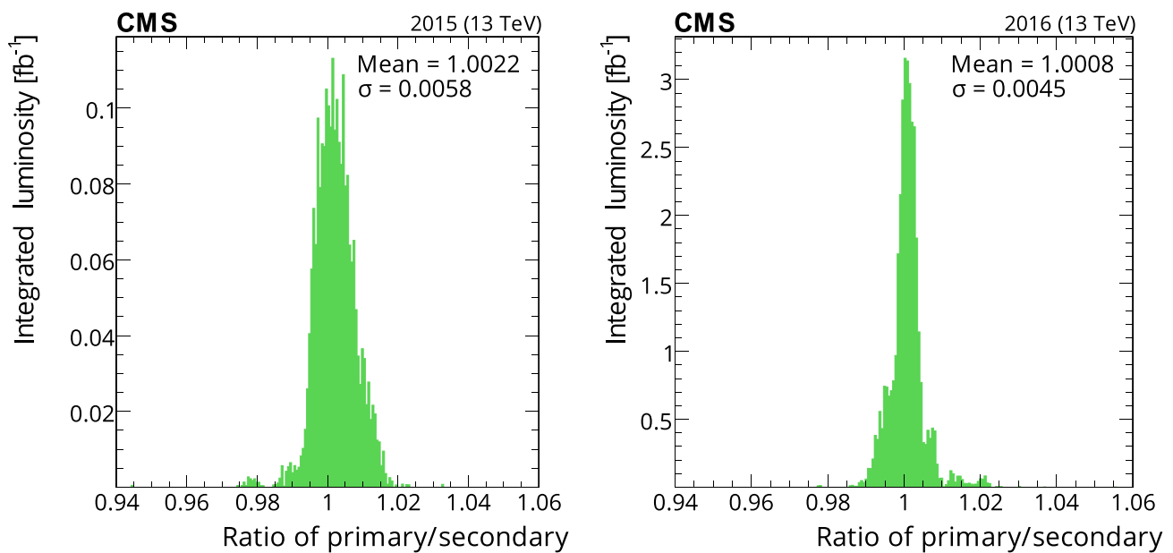
Fig. 18 The ratio of the primary (best available) to secondary (next-best available) luminosity as computed in time windows of approximately 20 min each. The left plot shows the 2015 results (principally
