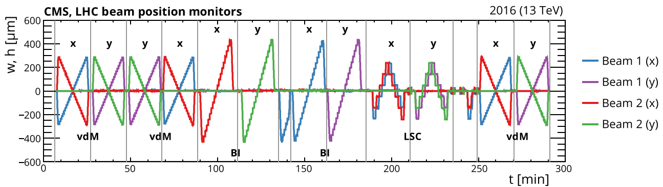
Fig. 3 Relative change in the positions of beams 1 and 2 measured by the DOROS BPMs during fill 4954 in the horizontal ( x ) or vertical ( y ) directions, as a function of the time elapsed from the beginning of the program. The gray vertical lines delineate vdM, BI, or LSC scans
