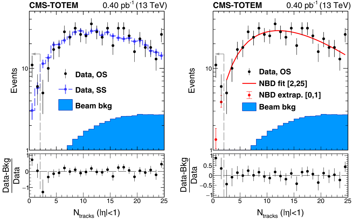
FIG. 7. Charged particle multiplicity distribution in the |\eta| < 1 region after the dijet and proton selection. Opposite side (OS) dijet events satisfy \eta^{\text{j}e\text{t}1}\eta^{\text{j}e\text{t}2} < 0 . The vertical bars represent the statistical uncertainties. The filled histogram represents the residual beam background contamination. The contribution of standard diffractive dijet events that feature a central gap is modeled with the same side (SS) dijet events (left) and with the negative binomial distribution (NBD) function fit (right), as described in the text. The NBD function is fit in the interval 2 \leq N_{\text{tracks}} \leq 25 , and extrapolated to N_{\text{tracks}} = 0 . The dashed-line arrow represents the region N_{\text{tracks}} < 2 used for signal extraction in the analysis. The vertical bars of the NBD extrapolation points represent the uncertainty in the extrapolation based on the fit parameter uncertainties extracted in the 2 \leq N_{\text{tracks}} \leq 25 interval.
