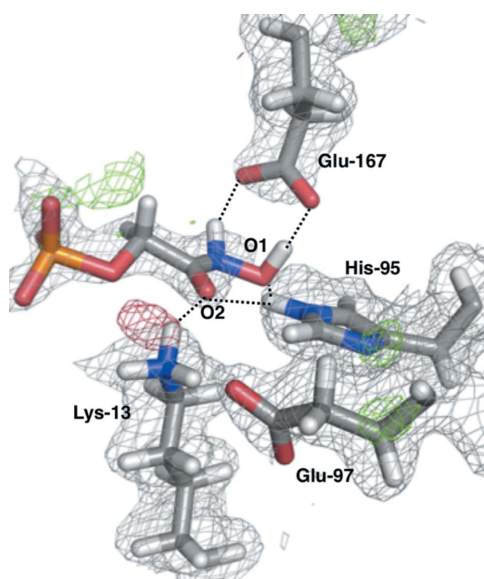
Figure 6 Quantum-refined joint X-ray/neutron structure of PGH–TIM with the 2mF - DF_c nuclear scattering-length density map contoured at 1.0\sigma and the mF_o - DF_c nuclear scattering-length difference density maps contoured at 3.0\sigma (green) and -3.0\sigma (red).
