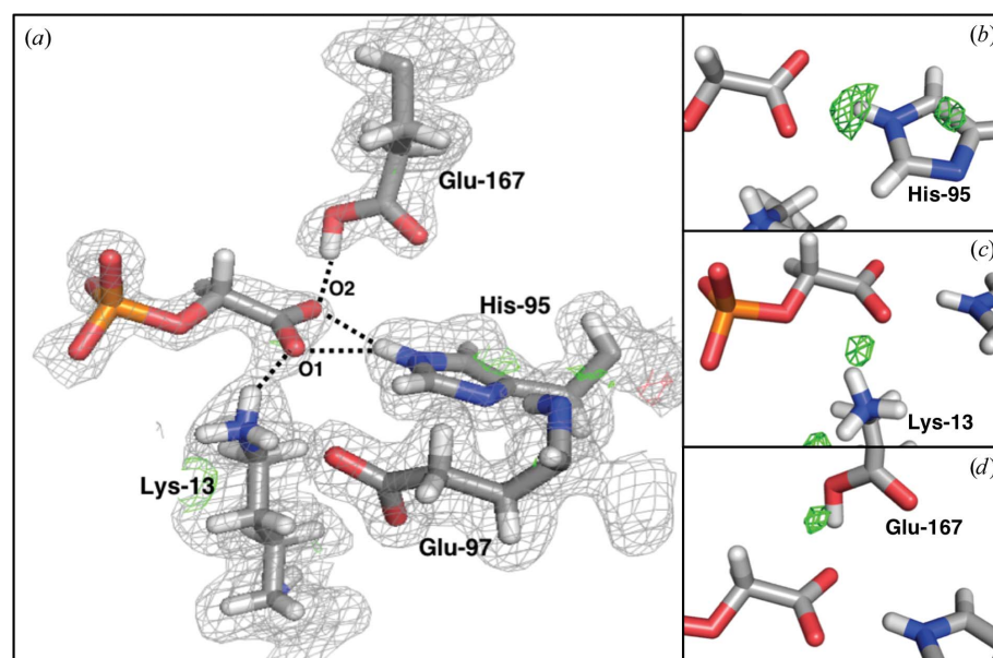
Figure 3 (a) Joint X-ray/neutron-refined structure of PGA–TIM with the 2mF_o - DF_c nuclear scattering-length density map contoured at 1.0\sigma and the mF_o - DF_c nuclear scattering-length difference density maps contoured at 3.0\sigma (green) and -3.0\sigma (red). (b–d) Nuclear scattering-length OMIT maps at 3.0\sigma of the D atoms of three important residues in the PGA–TIM active site: (b) His95, (c) Lys13 and (d) Glu167.
