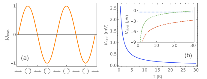
FIG. 3. Experimental signatures. (a) Magnon photocurrent as a function of polarization obtained by varying the angle between the electric field of a linearly polarized laser and the fast axis of a quarter wave plate. The resulting polarization is indicated below the graph. (b) Inverse spin Hall effect voltage V_{\text{ISHE}} induced by a magnon current as a function of temperature T . The main panel shows the diagonal Stokes component, while the inset shows the off-diagonal Stokes (blue, dotted), and diagonal (green, dashed) and off-diagonal (brown, dot-dashed) anti-Stokes contributions to V_{\text{ISHE}} . In both panels, the parameters are the same as in Fig. 2.
