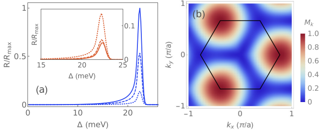
FIG. 4. Optical properties of honeycomb antiferromagnets. (a) Raman cross section as a function of \Delta = \hbar\omega_{\text{in}} - \hbar\omega_{\text{sc}} for a right-handed polarized laser at normal incidence (solid lines), and at incidence angles \theta = \pi/4 (dashed lines) and \theta = \pi/2 (dotted lines). The blue (orange) curves show the cross section for scattering into a left-handed (right-handed) photon. (b) Normalized Raman form factor M_{\mathbf{k}q_{\text{in}}} as a function of \mathbf{k} for a right-handed polarized laser at normal incidence. In all panels, the parameters are the same as in Fig. 2.
