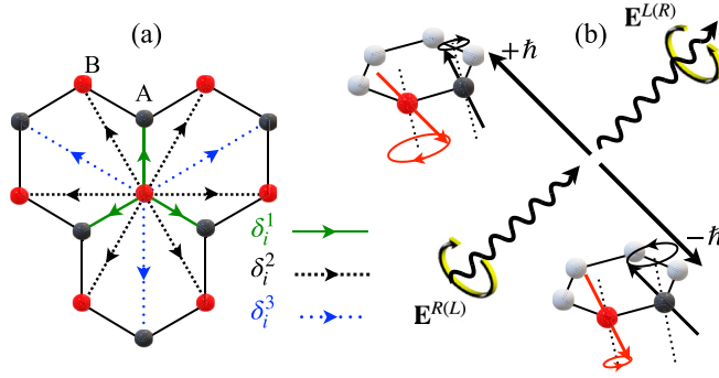
FIG. 1. Magnon photocurrent via two-magnon Raman scattering. (a) The magnetic unit cell with the vectors \delta_i^{(n)} connecting the n th-nearest neighbors. (b) Scattering of right-handed (left-handed) photons into left-handed (right-handed) photons imparting spin angular momentum and creating a magnon pair with zero net momentum carrying a net spin angular momentum current of 2\hbar
