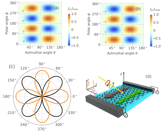
FIG. 2. Photoinduced magnon current. (a), (b) Photoinduced magnon current along the y axis as a function of incidence and polar angles \theta and \phi for left-handed (a) and right-handed (b) circular polarization. The current is normalized to the maximal value J_{\text{max}} obtained at \theta \approx 55^\circ and \phi = 45^\circ . The horizontal grid lines indicate where the incident field is parallel to the x or y axis. (c) The x component (orange) and y component (black) of the magnon photocurrent as a function of polar angle \phi . (d) Illustration of the proposed experimental setup with a honeycomb antiferromagnet and metallic contacts (Pt) for magnon current readout. In all panels, the model parameters are S = 5/2 , J_1 = 1.54 meV, J_2 = -0.14 meV, J_3 = 0.3 meV, J_z = 8.6 \mu eV, and B = 0 , as appropriate for MnPS 3 [36,37].
