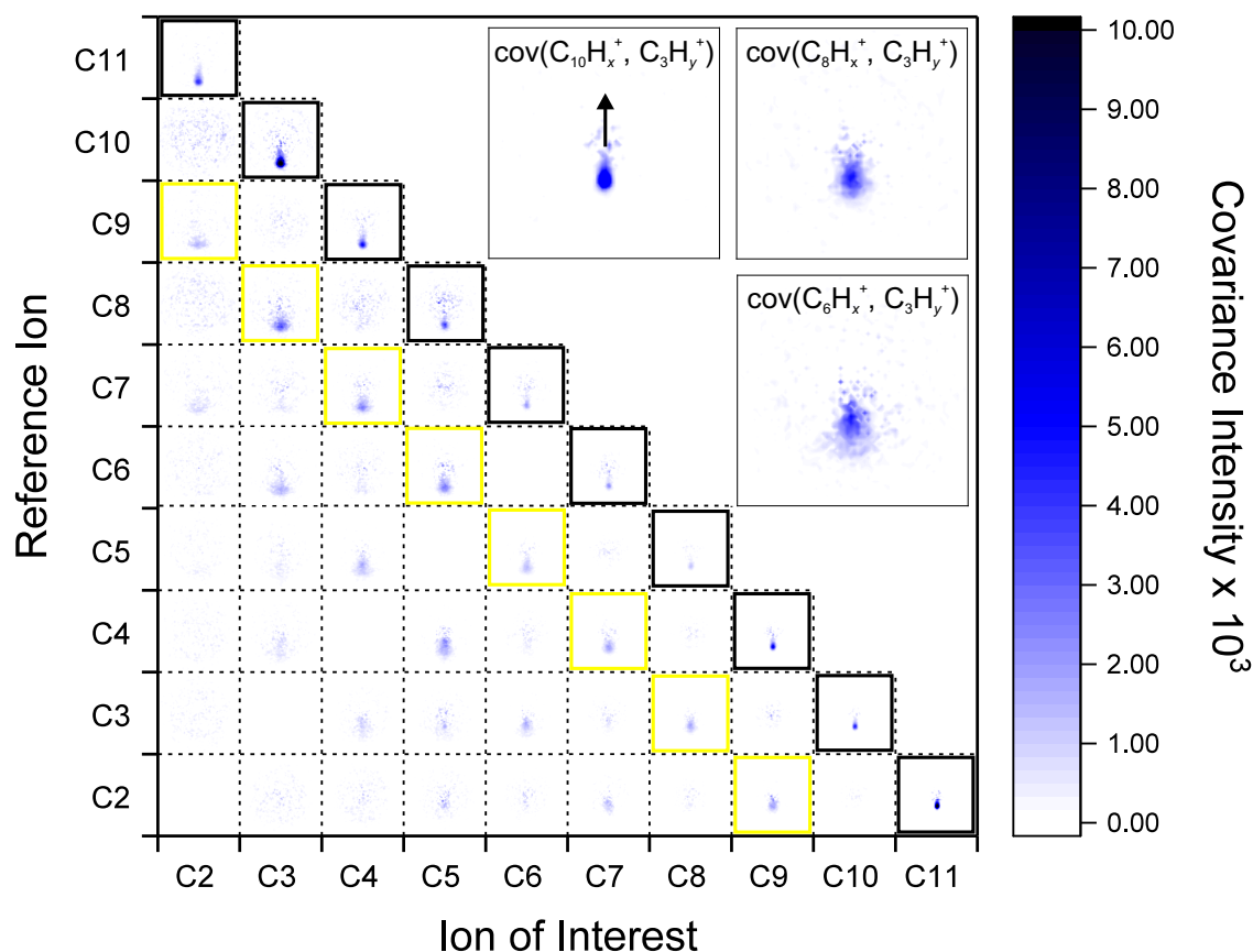
Figure 3. Full recoil-frame covariance map images. The covariance map images between all ion species produced from FLU. Axis labels refer to the number of carbons in the monocationic species and omit the number of hydrogen atoms. Fragment ion pairs that have a total number of carbons greater than that of the parent ion, for example, between C_8H_x^+ and C_9H_x^+ , show no covariance as they cannot be formed as partners from the same parent molecule; these have been omitted for clarity. Any ion species will also always show covariance with itself (autocovariance), and these entries have also been omitted. Notably, signal in the cells along the main diagonal of the matrix (highlighted in black) corresponds to the two-body dissociation pathways from the FLU^{2+} ion. Additionally, the cells highlighted in blue and red correspond to the dissociation pathways where two and four carbon atoms, respectively, are lost in neutral co-fragments. Inset: expansions for the maps corresponding to cov(C_{10}H_x^+, C_3H_y^+) , cov(C_8H_x^+, C_3H_y^+) , cov(C_6H_x^+, C_3H_y^+) showing increased blurring as more carbon atoms are lost in neutral co-fragments. The black arrow indicates the direction of the reference ion in all covariance maps.
