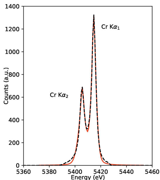
Figure 16 K\alpha fluorescence of a 5 \mu\text{m} Cr foil irradiated by an 10 \mu\text{m} X-ray FEL spot for calibration purposes (black-dashed) with fit (red). The spectral broadening of the lines by the 80 mm radius-of-curvature and 40 \mu\text{m} -thick HAPG crystal is \sim 2 eV. Reproduced from Preston et al. (2020).
