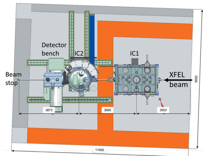
Figure 13 Floor plan of HED experiment hutch with the positions of IC1 (right, rectangular), IC2 (center, round) and the AGIPD on the detector bench on the left. The XFEL beam enters from the right. The dark-gray areas indicate hutch infrastructure, while the orange areas mark access paths. Dimensions are given in millimetres.
