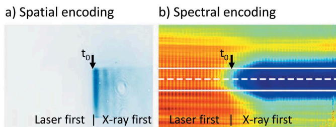
Figure 12 Typical images of PAM. (a) Spatial encoding: vertical versus horizontal position; time mapping results form an angle between the laser and the X-ray on the sample (2 \mu\text{m} -thick \text{Si}_3\text{N}_4 ). The temporal window (horizontal) is about 3.6 ps. (b) Spectral encoding image: lateral position versus the wavelength mapped to time by a chirped laser pulse collinear with the X-ray perpendicular to the sample (100 \mu\text{m} -thick YAG:Ce). The temporal window (horizontal axis of the image) is about 1.7 ps. Both show a shadow due to the X-ray-induced opacity change of the sample. At t_0 both beams are timed. The horizontal edges in (a) result from the upstream partially closed power slits which are not influencing (b).
