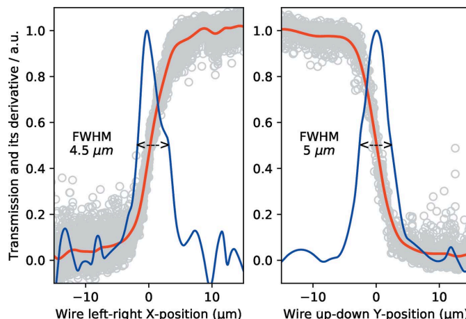
Figure 8 Characterization of the best focus of CRL3 after intermediate focus with CRL1 at 17.8 keV with a wire scan. The scans took a few minutes with 5% transmission. The y-axis shows in red the transmission (normalized to the incident pulse energy, and with a moving average), as well as its derivative in blue.
