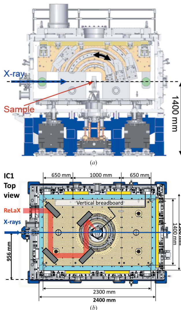
Figure 14 (a) Cut through the schematic of the IC1 target chamber showing the vertical breadboard with circular rails. (b) Top view of the interior of IC1; the access doors are at the bottom. In red, a typical beam path for the ReLaX laser is shown, and the back line indicates a sample viewing system. The beam transport of the DiPOLE-100X high-energy laser in IC1 is flexible and customized configurations are currently evaluated.
