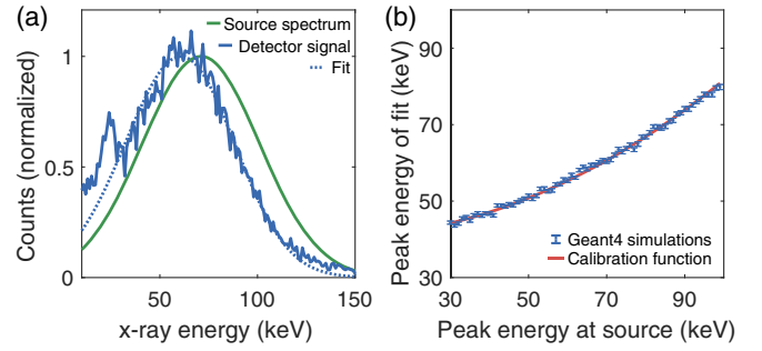
FIG. 2. Simulation of x-ray transport and detection. (a) An x-ray source spectrum (green), the detector signal of this x-ray beam (solid blue), and the double Gaussian fit used to determine the peak of the deposited energy distribution (dotted blue). (b) Peak of the detector signal and 68% confidence intervals from fitting routine as a function of the peak energy of the source spectrum (blue). The calibration function (red) is used for the adjustment of measured data.
