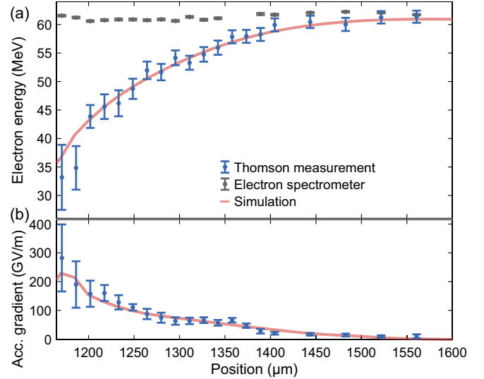
FIG. 4. (a) Electron beam energy measured via Thomson scattering as function of the overlap position (blue). The final electron beam energy at each interaction point is shown as the average peak of Gaussian fits to the single electron spectra with its standard error (gray). The energy evolution obtained from the PIC simulation is shown as a red line, for better comparison again using Gaussian fits. (b) Acceleration gradient as function of the overlap position. The acceleration gradient was calculated using a linear fit of \pm 3 data points. At the edges only available data points were included. The error bars display the 68% confidence interval.
