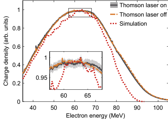
FIG. 3. Normalized electron spectrum of 340 shots with Thomson laser turned on at an overlap position of 1330 \mu\text{m} (gray line), the standard error from individual normalized shots (gray area) and the normalized electron spectrum at the same overlap position without the Thomson laser (orange dashed line). The error band without the Thomson laser is similar to the displayed band with the Thomson laser activated. The same level of agreement between signal and background shots was also observed at overlap positions of 1190 \mu\text{m} and 1560 \mu\text{m} . The region around the peak is shown in more detail in the inset. The spectrum obtained from PIC simulations is depicted as a red dotted line. All lines are normalized individually.
