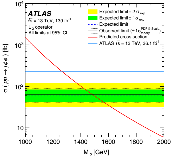
FIG. 9. Observed (solid line) and expected (dashed line) exclusions at 95% CL on the Horndeski dark-energy model for m_\phi = 0.1 GeV and c_{i \neq 2} = 0, c_2 = 1 [6], expressed in terms of the visible cross section as a function of the suppression scale M_2 . The results are compared with the theoretical predictions. The dotted lines around the observed limits indicate the range of observed limits corresponding to \pm 1\sigma variations of the cross-section predictions. The results from this analysis are compared with previous results from the ATLAS Collaboration at \sqrt{s} = 13 TeV using 36.1 fb -1 [6].
