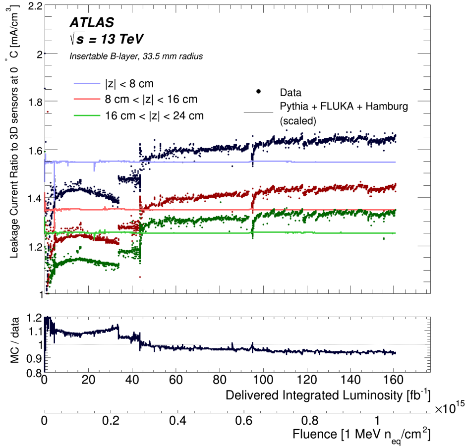
Figure 5. The measured and predicted leakage currents on the Insertable B -layer, both normalized to 0 °C, divided by the currents in the 3D modules at 24 < |z| < 32 \text{ cm} . The other three module groups represent |z| < 8 \text{ cm} , 8 < |z| < 16 \text{ cm} , and 16 < |z| < 24 \text{ cm} . The A and C sides of the detector ( z > 0 and z < 0 ) are consistent with each other and averaged. The dominant time-independent uncertainty of 10% is not included to avoid overlapping bands. The prediction is based on the thermal history of the modules combined with the Hamburg Model for modelling changes in the leakage current and PYTHIA + FLUKA for simulating the overall fluence. For all four predictions, the overall scale normalization is based on a fit to the data across the entire range. Normalization factors are determined per |z| region. The lower panel shows the ratio of the prediction to the data for the innermost module group. Similar MC/data trends are observed for the other three |z| regions. For illustration, the fluence is shown as a lower horizontal axis using the nominal luminosity-to-fluence from simulation at |z| = 0 .
