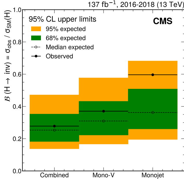
Figure 6: Upper limits at 95% CL on the branching fraction B of the Higgs boson to invisible final states. The results are shown separately for the monojet and mono-V categories, as well as for their combination. The final combined limit is 27.8% (25.3% expected).
