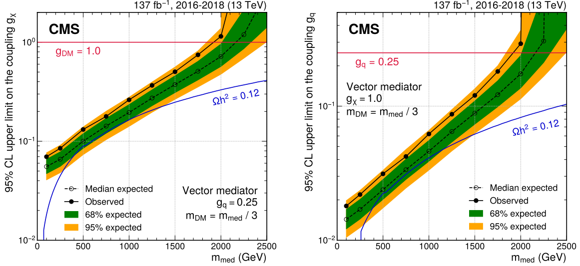
Figure 20: Exclusion limits at 95% CL on the couplings g_\chi (left) and g_q (right) for a vector mediator. In each panel, the result is shown as a function of the mediator mass m_{\text{med}} , and the mass of the DM candidate is fixed to m_{\text{DM}} = m_{\text{med}}/3 . In either case, only one coupling is varied, and the respective other coupling is fixed at its default value ( g_q = 0.25 , g_\chi = 1.0 ). The blue solid line indicates the parameter combinations for which the simplified model reproduces the observed DM relic density. Around m_{\text{DM}} \approx m_{\text{top}} , corresponding to m_{\text{med}} \approx 500 GeV, DM annihilation into top quarks becomes possible, leading to a shift in the relic density.
