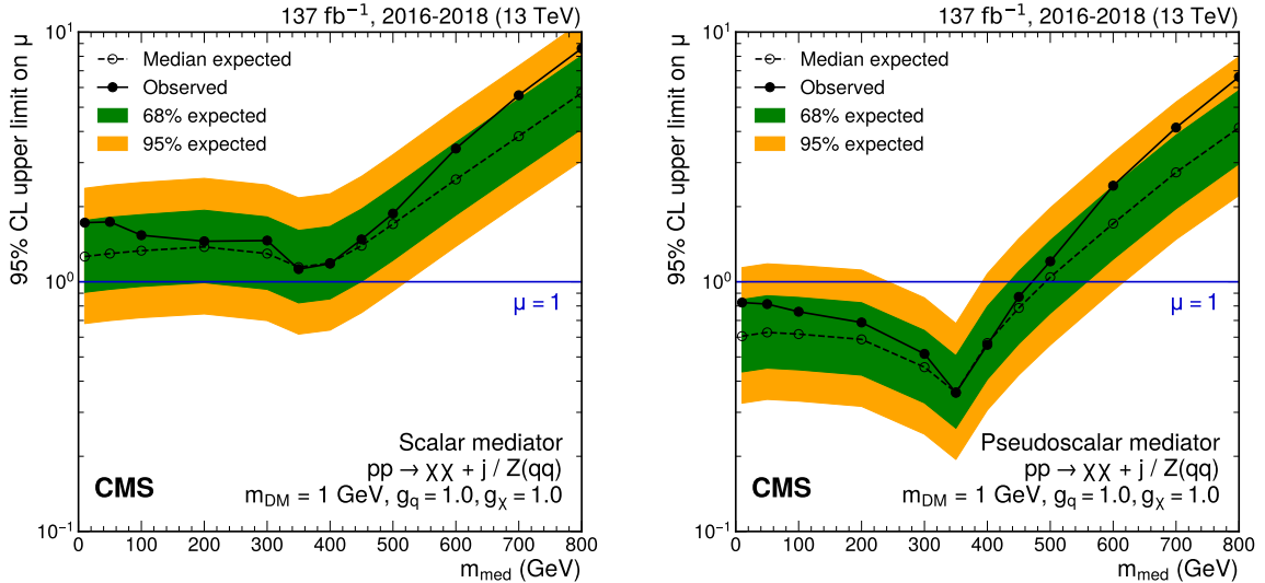
Figure 9: Upper limits at 95% CL on the signal strength \mu = \sigma / \sigma_{\text{theo}} as a function of m_{\text{med}} for scenarios with scalar (left) and pseudoscalar (right) mediators and coupling values of g_q = 1.0 , g_\chi = 1.0 , for a constant value of m_{\text{DM}} = 1 \text{ GeV} . The blue solid line indicates the exclusion boundary \mu = 1 . In the case of a pseudoscalar mediator, m_{\text{med}} values up to 470 GeV are excluded (490 GeV expected).
