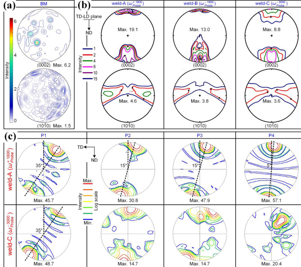
Fig. 3. The (0002) and (1010) PFs showing macrotexture of (a) BM and (b) SZ of weld-A, B and C. (c) (0002) PF of P1-4 positions illustrated in Fig. 2(c). Note that the initial macrotexture of BM was examined by X-ray diffraction. To obtain grain statistics, an area of 100 \times 50 \text{ mm}^2 was scanned.
