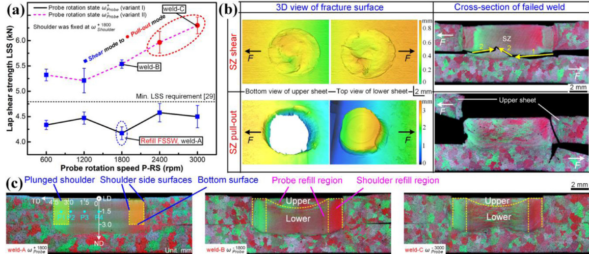
Fig. 2. (a) LSS and fracture mode for different probe rotation states, the shoulder rotation state is fixed at \omega_{Shoulder}^{+1800} , thus \omega_{Probe}^{+} and \omega_{Probe}^{-} correspond to the variant I and II of DR-refill FSSW, respectively. (b) Illustrations of failure modes: SZ shear and pull-out mode. (c) Cross-sectional macrostructures of weld-A, B and C. The experimental coordinate system is defined by normal direction (ND), transverse direction (TD) and longitudinal direction (LD) as shown in (c).
