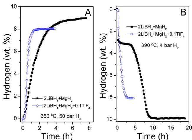
Figure 2. (A) Second hydrogenation and (B) second dehydrogenation for 2\text{LiBH}_4 + \text{MgH}_2 and 2\text{LiBH}_4 + \text{MgH}_2 + 0.1\text{TiF}_4 hydride systems. Isothermal hydrogenation/dehydrogenation at 350\text{ }^\circ\text{C} under 50\text{ bar H}_2 and 390\text{ }^\circ\text{C} under 4\text{ bar H}_2 , respectively.
