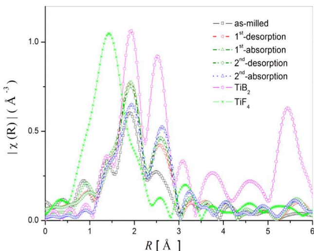
Figure 4. Fourier transformation of the EXAFS function in the k -range of [0–6] Å -1 of Ti-containing hydride matrix at different hydrogenation cycles together with the reference spectra.
