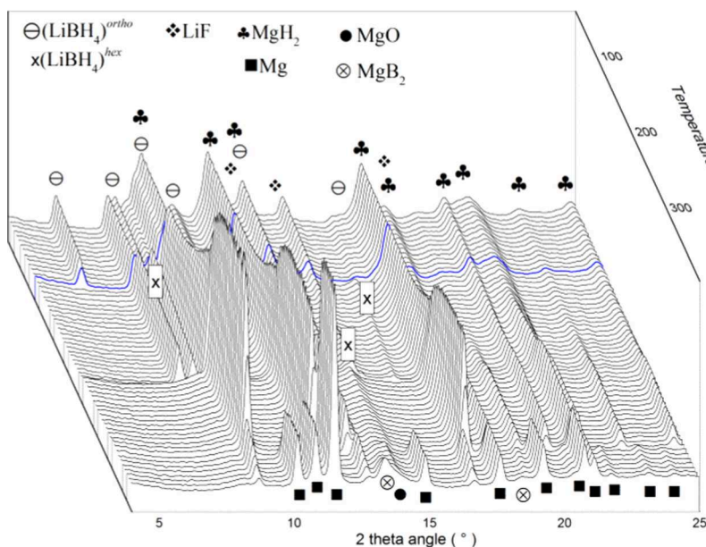
Figure 3. In situ SR-XPD for the first dehydrogenation reaction of 2\text{LiBH}_4 + \text{MgH}_2 + 0.1\text{TiF}_4 under 4\text{ bar H}_2 backpressure. The temperature was increased with a ramp of 3\text{ }^\circ\text{C/min} from RT to a maximum temperature of 400\text{ }^\circ\text{C} .
