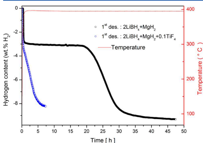
Figure 1. First nonisothermal dehydrogenation reaction from room temperature (RT) to 400 °C, heating rate 3 °C/min, and under \text{P}_{\text{H}_2} = 4 bar \text{H}_2 dehydrogenation for 2\text{LiBH}_4 + \text{MgH}_2 and 2\text{LiBH}_4 + \text{MgH}_2 + 0.1\text{TiF}_4 hydride systems.
